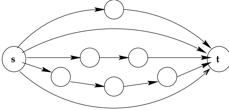
Figure 3: Worst-case networks for inhomogeneous sets of cost functions. The number of paths and the number of edges in each path can be arbitrarily large.
