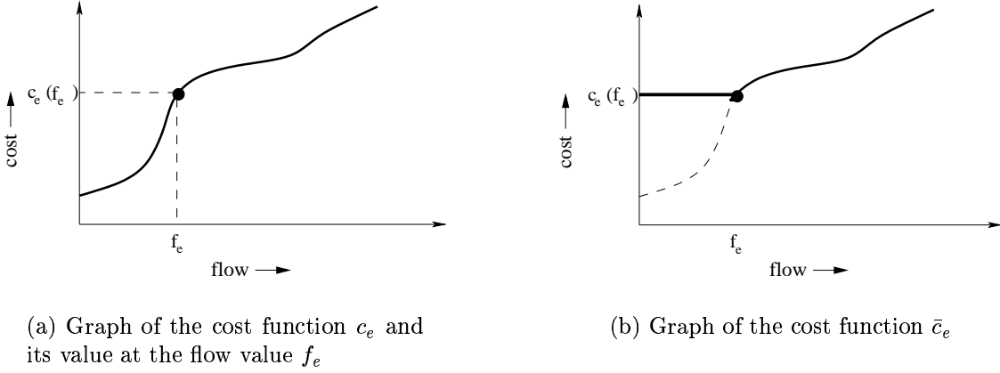
Figure 7: Construction in the proof of Theorem 4.2 of the modified cost function \bar{c}_e given the original cost function c_e and the Wardrop equilibrium value f_e . Solid lines denote graphs of functions.
