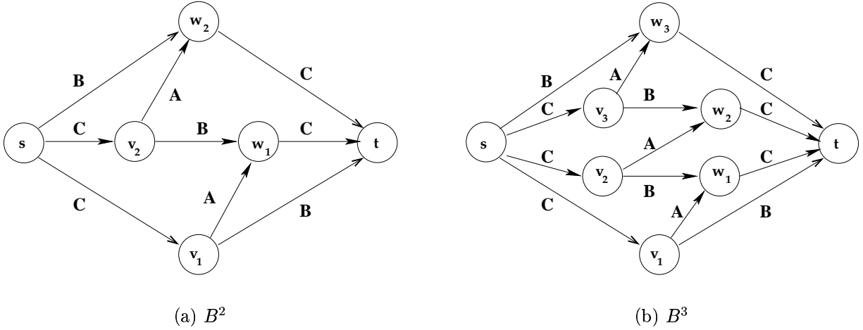
Figure 4: The second and third Braess graphs. Edges are labeled with their types.
