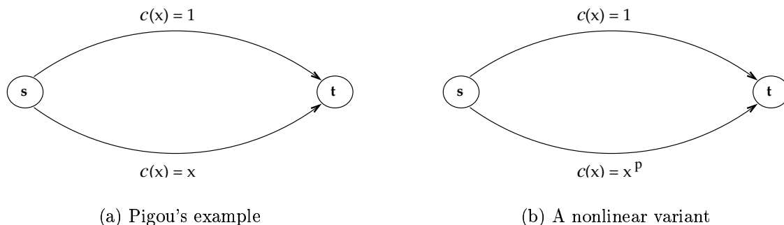
Figure 1: Pigou's example and a nonlinear variant. The cost function c(x) describes the cost incurred by users of an edge, as a function of the amount of traffic routed on the edge.
