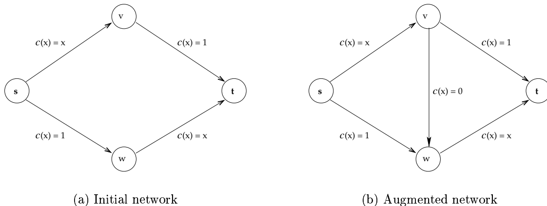
Figure 2: Braess’s Paradox. The addition of an intuitively helpful edge can adversely affect all of the traffic.
