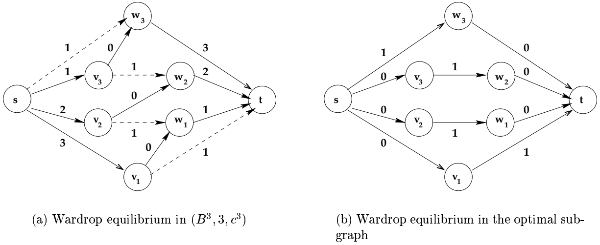
Figure 5: Proof of Theorem 3.4, when k = 3 . Solid edges carry traffic in the Wardrop equilibrium, dashed edges do not. Edge costs are with respect to the Wardrop equilibrium.
