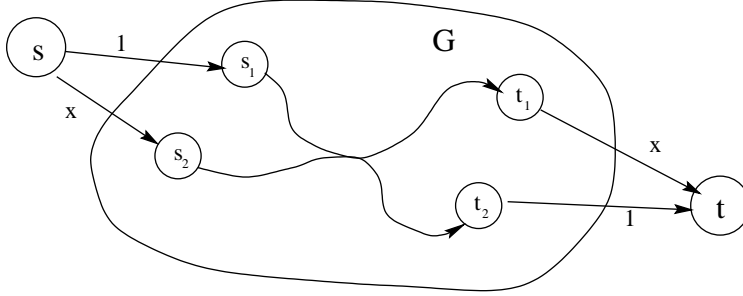
Figure 6: Proof of Theorem 3.21. In a “no” instance of 2DDP, the existence of s_1-t_1 and s_2-t_2 paths implies the existence of an s_2-t_1 path.
