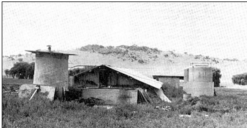
Fig. 32 Digester with storage tank in background
