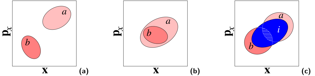
Figure 8: Convergence of an FEP calculation. If the ensembles representative of states a and b are too disparate, equation (59) will not converge (a) . If, in sharp contrast, the configurations of state b form a subset of the ensemble of configurations characteristic of state a , the simulation is expected to converge (b) . The difficulties reflected in case (a) may be alleviated by the introduction of mutually overlapping intermediate states that connect a to b (c) . It should be mentioned that in practice, the kinetic contribution, \mathcal{T}(\mathbf{p}_x) , is assumed to be identical for state a and state b .
