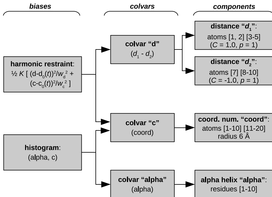
Figure 6: Graphical representation of a collective variables configuration. The colvar called “ d ” is defined as the difference between two distances: the first distance ( d_1 ) is taken between the center of mass of atoms 1 and 2 and that of atoms 3 to 5, the second ( d_2 ) between atom 7 and the center of mass of atoms 8 to 10. The difference d = d_1 - d_2 is obtained by multiplying the two by a coefficient C = +1 or C = -1 , respectively. The colvar called “ c ” is the coordination number calculated between atoms 1 to 10 and atoms 11 to 20. A harmonic restraint is applied to both d and c : to allow using the same force constant K , both d and c are scaled by their respective fluctuation widths w_d and w_c . A third colvar “alpha” is defined as the \alpha -helical content of residues 1 to 10. The values of “ c ” and “alpha” are also recorded throughout the simulation as a joint 2-dimensional histogram.
