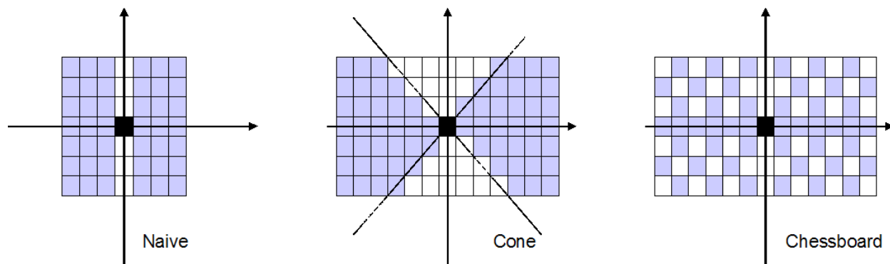
Figure 7. FIFO Mapping Schemes
