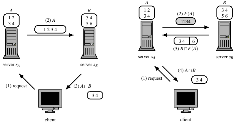
(a) A simple approach to “AND” queries. Each server stores a list of document IDs corresponding to one keyword.
