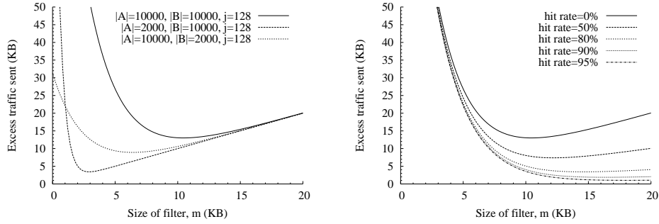
(a) Expected excess bits sent as a function of m
