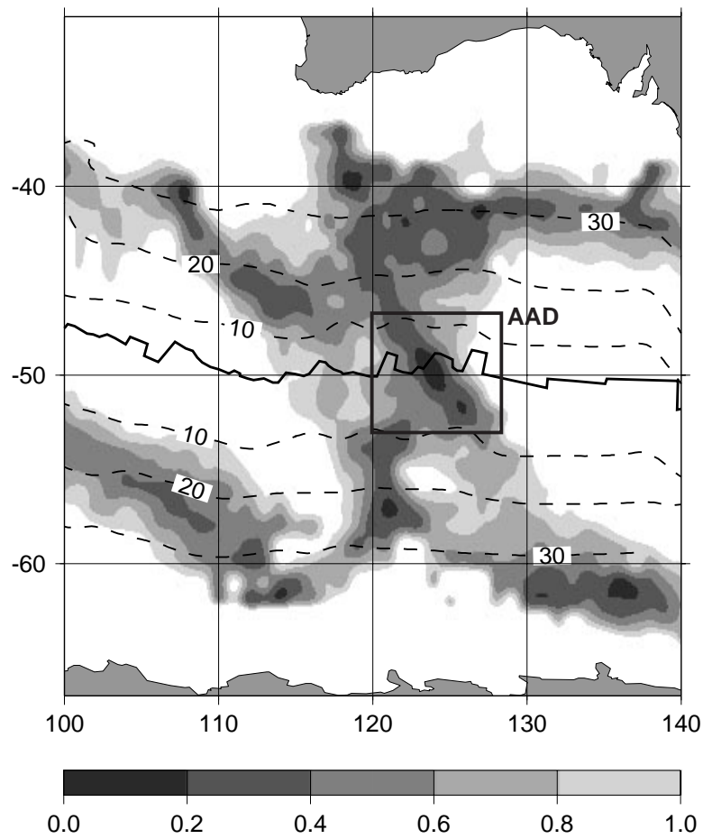
Figure 7. Similarity, defined by equation (1), between the mantle model beneath the starred point in Figure 1 and the rest of the southeast Indian Ocean upper mantle. Darker grey shades indicate stronger similarity to the mantle beneath the AAD. Lithospheric age isochrons are shown as dashed lines.
