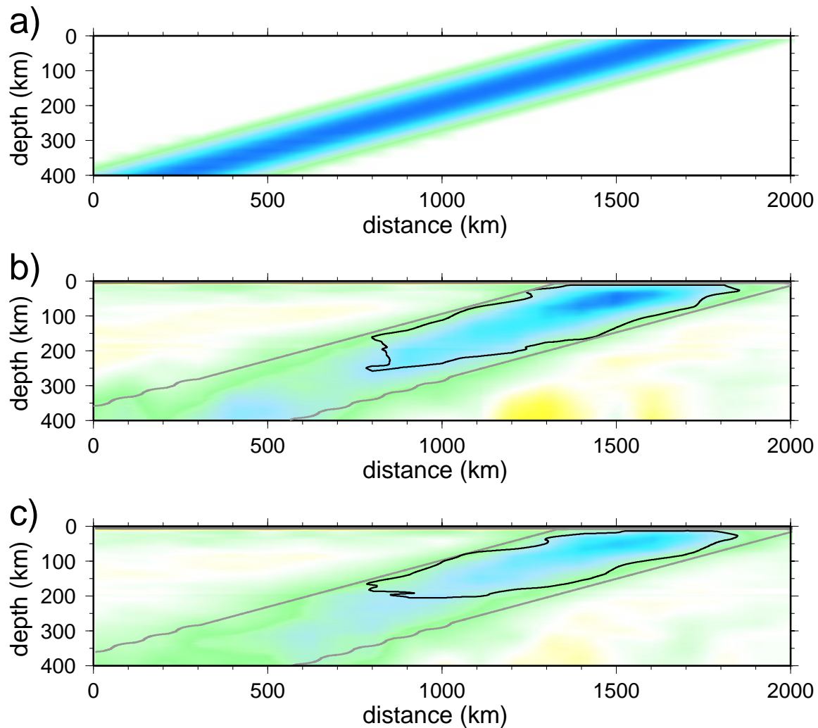
Figure 6. Synthetic resolution test. (a) Synthetic input model of a high velocity anomaly extending into the transition zone. This perturbation is taken relative to the 1 Ma age model. (b) Model estimated with the Monte-Carlo inversion of the synthetic phase and group velocities computed from the model in (a). (c) Model estimated from synthetic phase and group velocity maps that have been smoothed laterally to match the estimated resolution (Figure 2b). The color palette is the same as in Figure 5. The black contours indicate the persistent features in the inversion and the grey contours mark the outline of the input anomaly.
