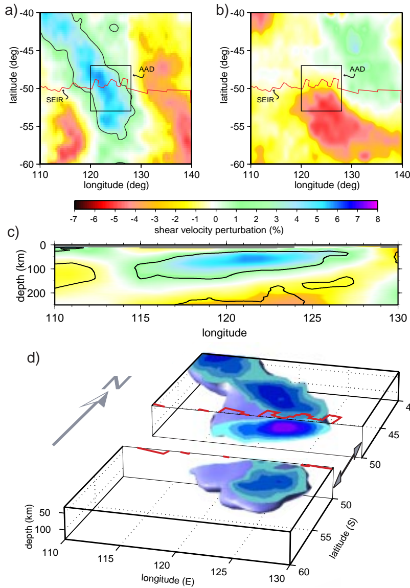
Figure 5. Images of the AAMA. (a) Horizontal slice of the V_s model at 60 km depth plotted with respect to the age-dependent model, some age profiles of which are shown in Figure 4. Black contours indicate +3% perturbations. (b) Similar to (a), but at 200 km depth. (c) Vertical slice of the V_s model along path A - A' (Figure 1) relative to the 1 Ma age average. Black contour shows the persistent features of the model. (d) Isosurface (+2%) representation of the AAMA relative to the age-dependent model. The model was spatially smoothed to highlight the dominant large-scale features, which trend in the NW-SE direction and extend no deeper than about 120 km.
