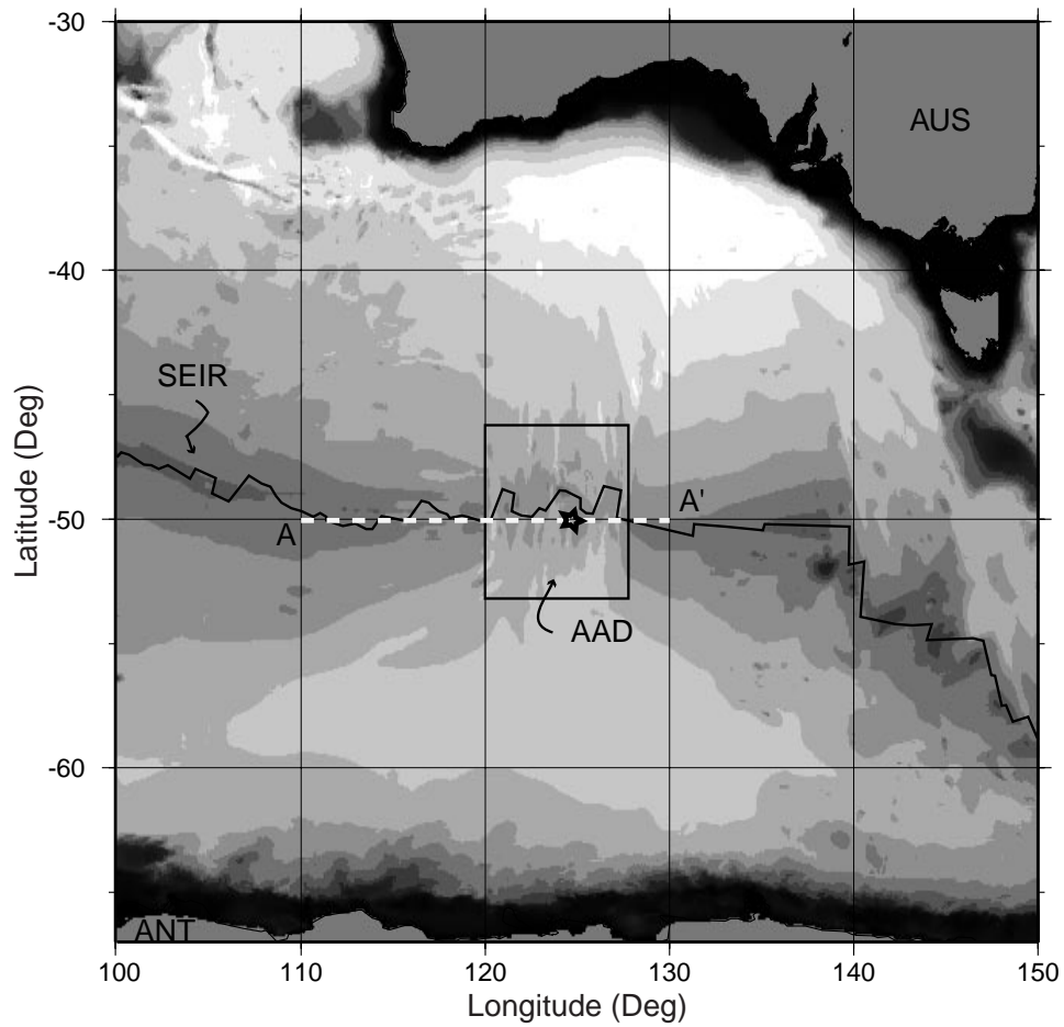
Figure 1. Bathymetric reference map of the Southeast Indian Ocean. The Australian-Antarctic Discordance (AAD) region is boxed. The Southeast Indian Ridge (SEIR) cuts across the center of the figure. The star ( 50^{\circ}\text{S} , 124^{\circ}\text{E} ) marks the location of the 1-D model shown in Figures 3b and 4.
