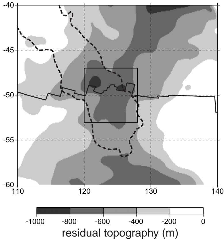
Figure 11. Residual topography ( dh ) compared with the 3% contour (dashed line) of the AAMA at 60 km depth (taken from Figure 5a). Residual topography is the difference between the observed topography (Smith and Sandwell, 1997) and topography predicted from sea floor age A in Ma: dh = 2620 \text{ m} - 350 \sqrt{A} \text{ m} . Both the observed and residual topography are smoothed using a spatial gaussian filter with a standard deviation of 70 km. The observed topography is corrected isostatically for sedimentary load taken from the crustal model of Laske and Masters (2002, personal communication). The residual depth anomaly (dark grey shades) forms a V-shaped feature that is poorly correlated with the AAMA except at the SEIR.
