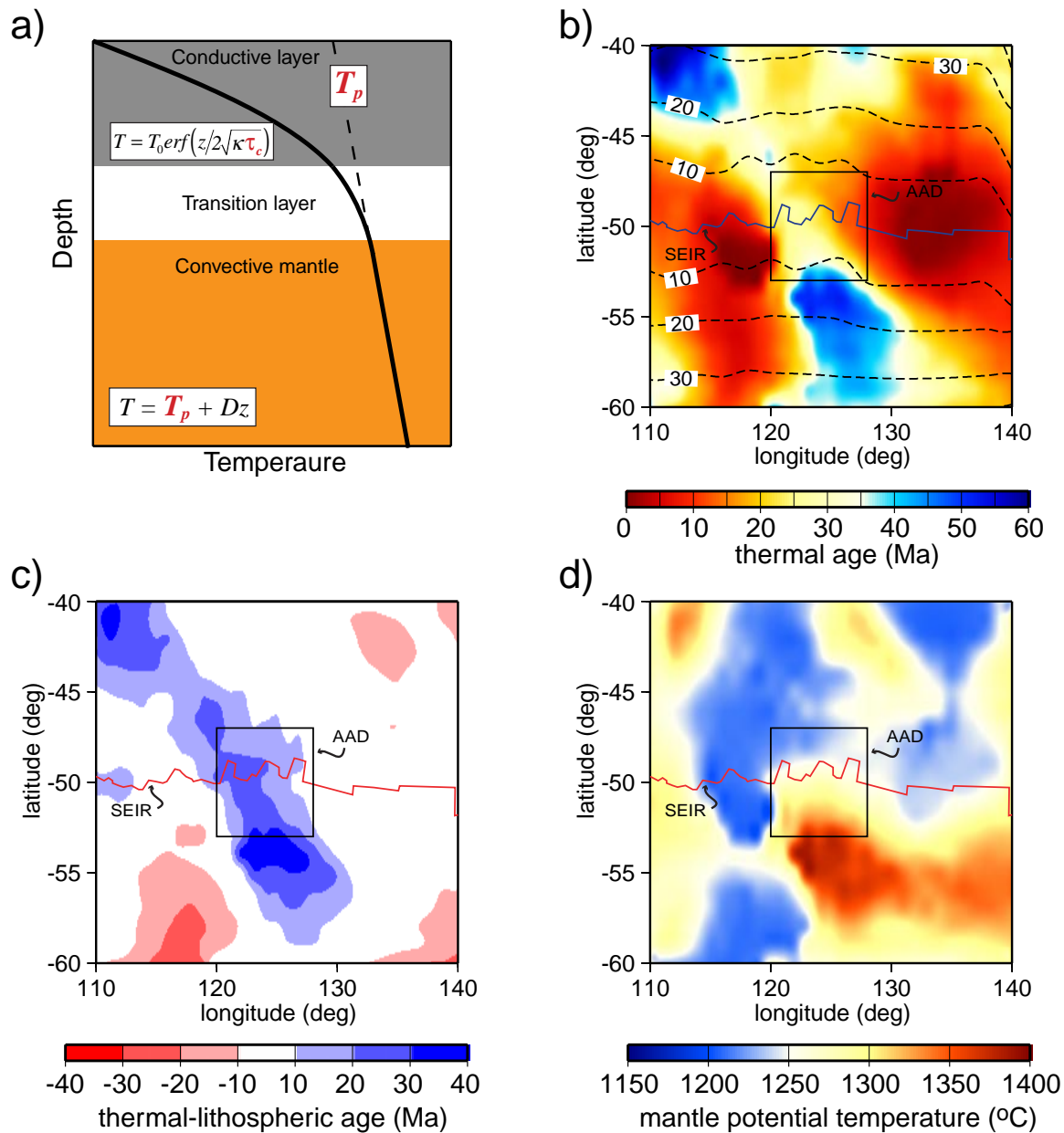
Figure 8. (a) Thermal parameterization of the oceanic lithosphere in which a conductive layer, described by thermal age \tau_c , is underlain by a convecting asthenosphere, described by potential temperature T_p . (b) Estimated apparent thermal age, \tau_c , across the southeast Indian ocean lithosphere. Isochrons of lithospheric ages are overplotted as dashed lines. (c) Difference between thermal age and lithospheric age. The entire AAMA, including the region of the AAD, is much cooler than its lithospheric age would suggest. (d) Estimated mantle potential temperature, T_p , of the southeast Indian ocean asthenosphere.
