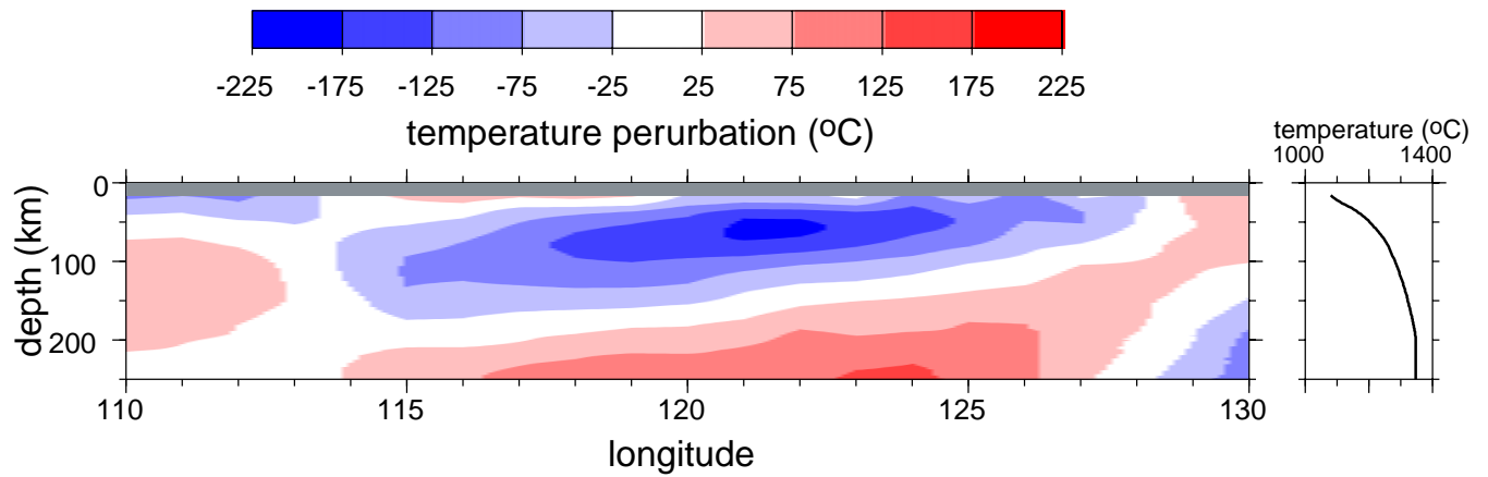
Figure 9. Temperature variations beneath profile A – A' in Figure 1, taken relative to the average temperature profile along the SEIR, shown at right.
