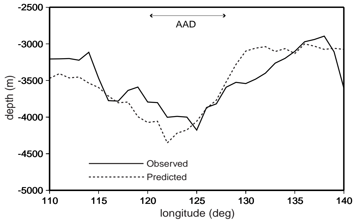
Figure 10. Comparison between the observed topography along profile A – A' in Figure 1 and that predicted assuming isostatic compensation from the temperature model shown in Figure 9.
