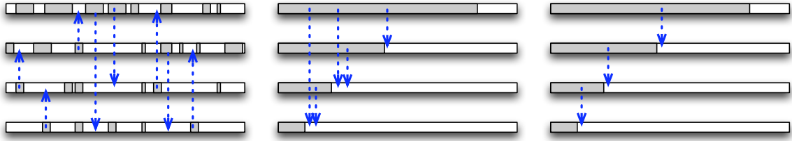
(a) Rarest Random : peers download rare chunks, becoming useful to the others despite having few chunks (b) Naive Sequential : peers with fewer chunks can get help from those with more but not vice versa, which makes chunks near the start have more sources. (c) Cascading : peers only download from a subset of neighbors and a chain is formed to propagate chunks.
