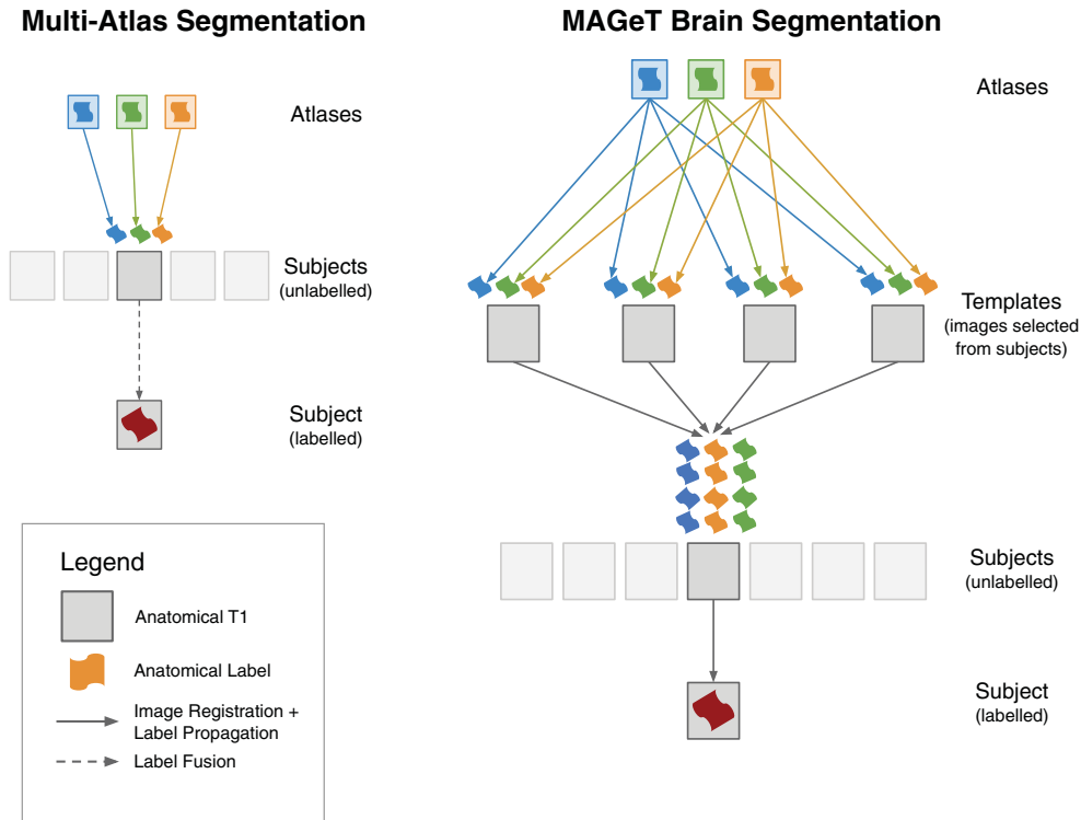
Fig. 1. A schematic illustration of basic multi-atlas segmentation and MAGeT-Brain segmentation. In multi-atlas segmentation, manual labels from atlas images are warped (propagated) into subject space by applying the transformations estimated from nonlinear image registration. The resulting candidate labels from all atlas images are then fused to create a final segmentation. In MAGeT-Brain segmentation, a template library is created by sampling (either randomly or representatively) from the subject images. Atlas labels are propagated to all template images and then to each subject image (including those used in the template library). The candidate labels for a subject are then fused into a final segmentation.
