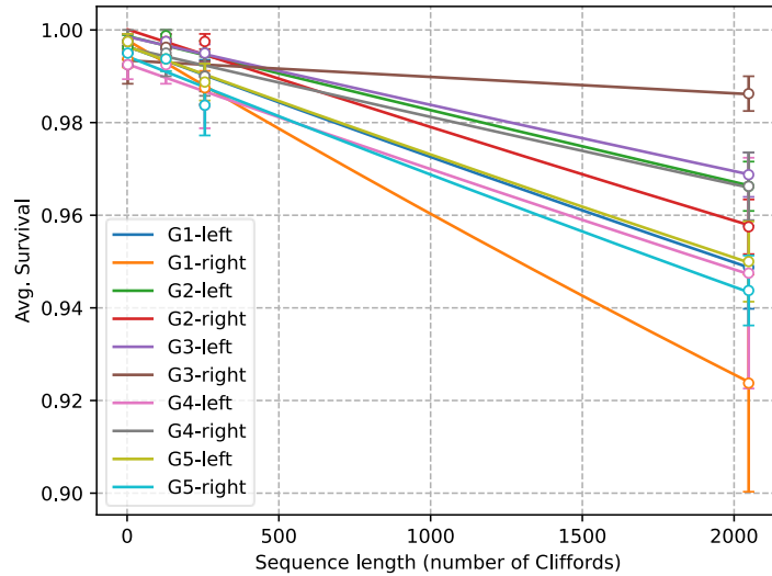
Figure 3 Single-qubit RB data from H1-1 taken on 2024/04/10 with 2 qubits per each of the 5 gate zones. Infidelity estimate averaged over all zones is 2.1(3) \times 10^{-5} .
