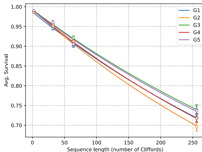
Figure 4: Two-qubit RB results from H1-1 taken on 2024/04/10. Infidelity estimate averaged over all 5 zones is 8.8(3) \times 10^{-4} .
