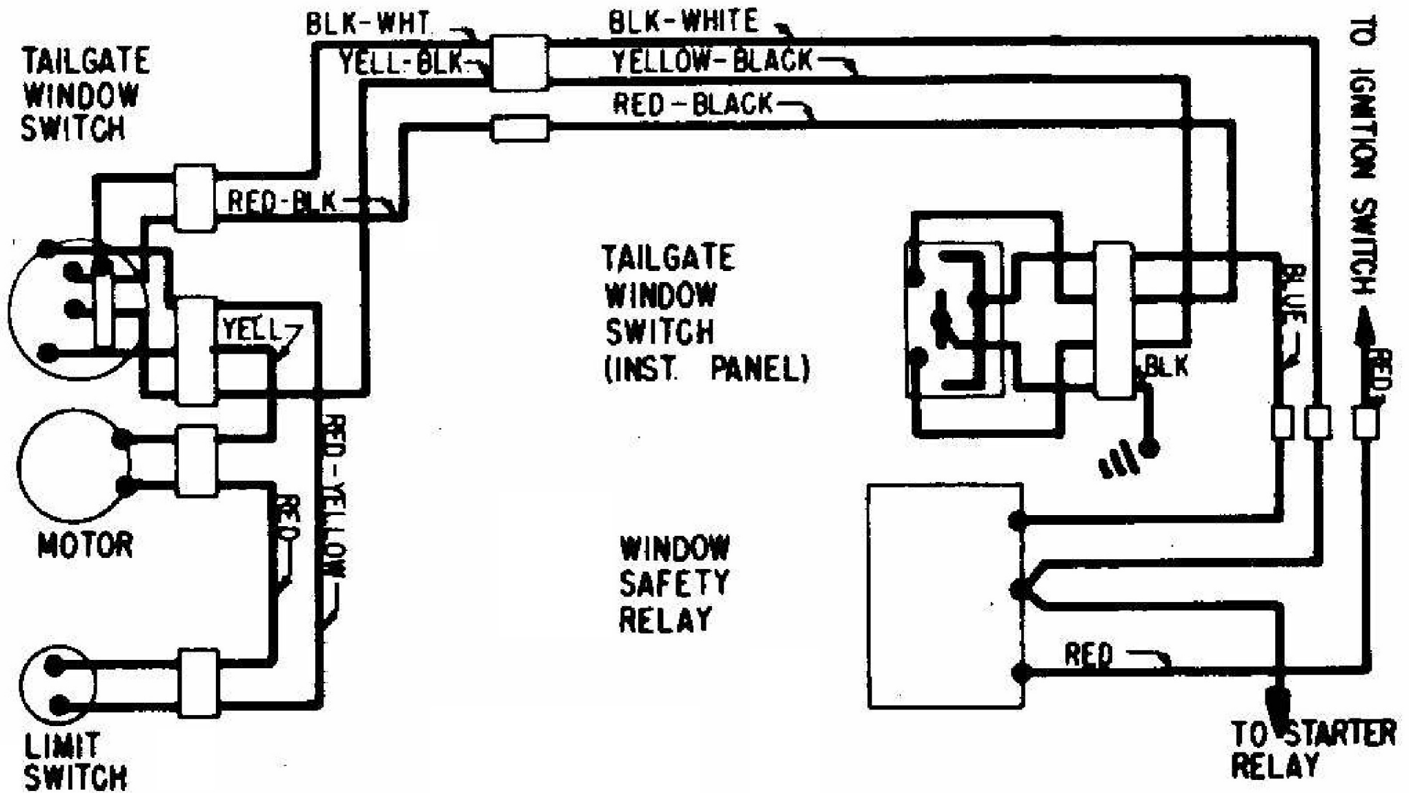
TYPICAL TAILGATE WIRING DIAGRAM
