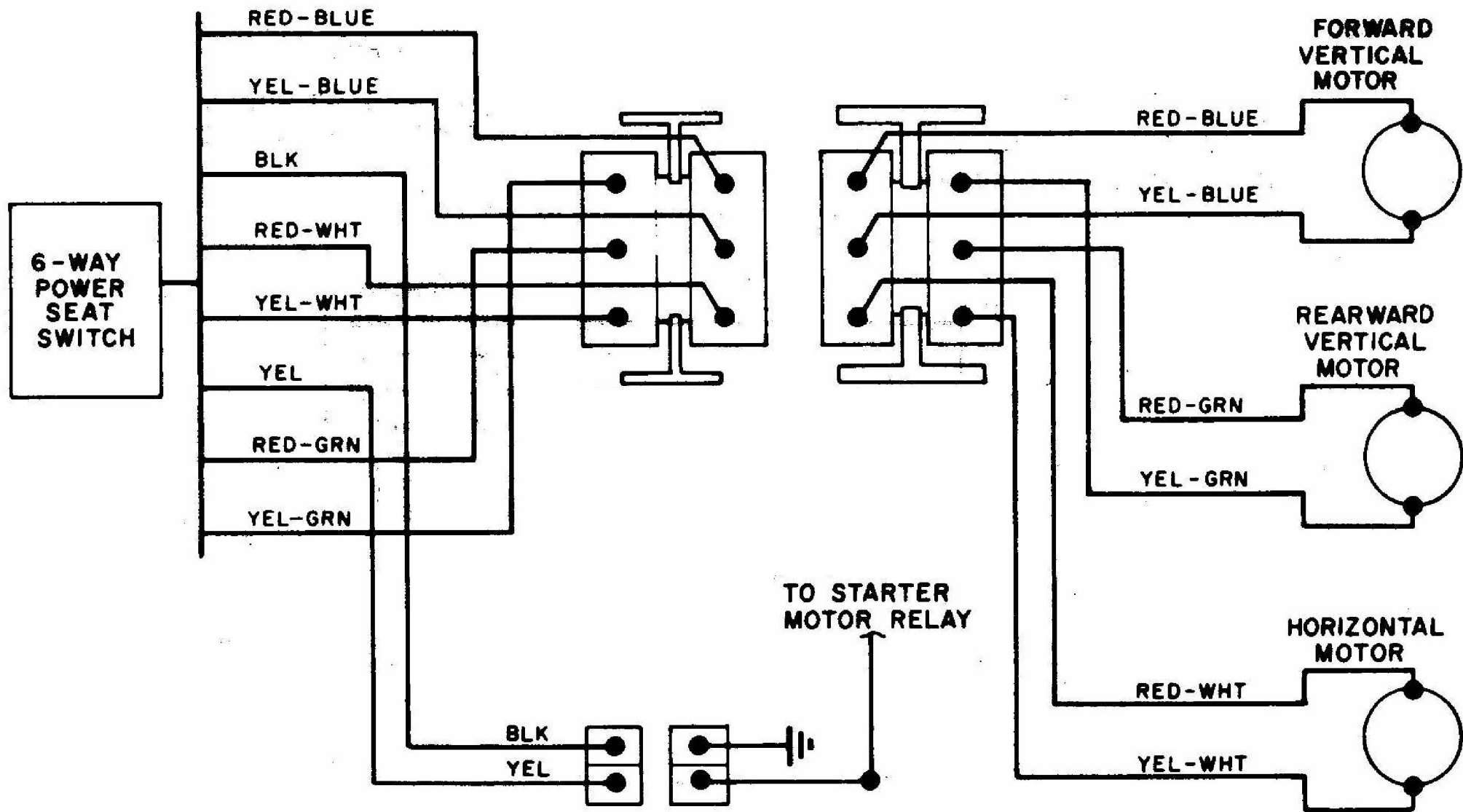
FORD 6-WAY WIRING DIAGRAM
