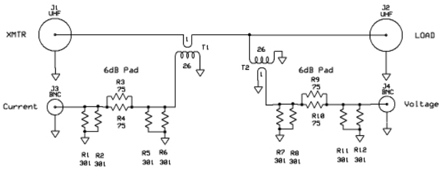
Coupler Schematic
