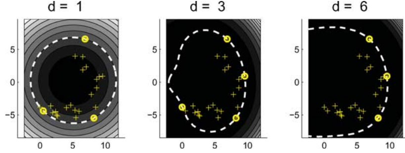
Figure 2. Data description trained on a banana shaped data set. Kernel is a polynomial kernel with varying degrees. Support vectors are indicated by the solid circles, the dashed line is the description boundary.
