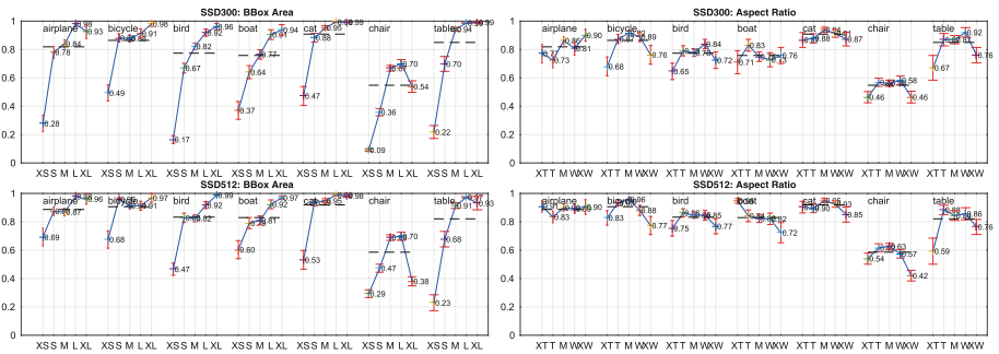
Fig. 4. Sensitivity and impact of different object characteristics on VOC2007 test set using [19]. The plot on the left shows the effects of BBox Area per category, and the right plot shows the effect of Aspect Ratio.
