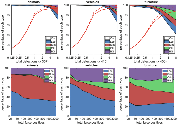
Fig. 3. Visualization of performance for SSD 512 on animals, vehicles, and furniture from VOC2007 test using [19]. The top row shows the cumulative fraction of detections that are correct (Cor) or false positive due to poor localization (Loc), confusion with similar categories (Sim), with others (Oth), or with background (BG). The bottom row shows the distribution of top-ranked false positive types.
