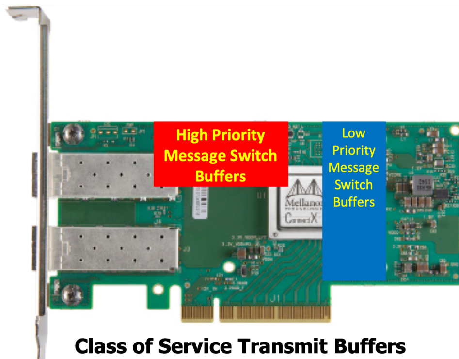
Figure 5: Class of Service Transmit Buffers on Mellanox ConnectX-5
