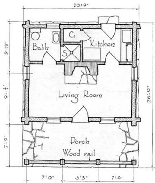
FLOOR PLAN Scale \frac{3}{32} " = 1'-0"
