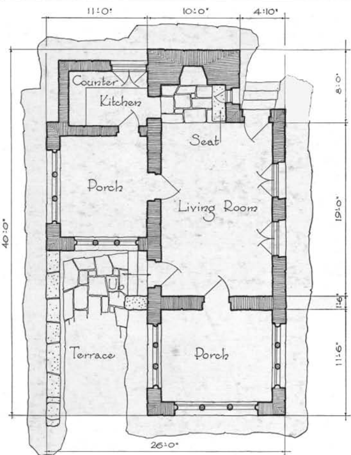
FLOOR PLAN
