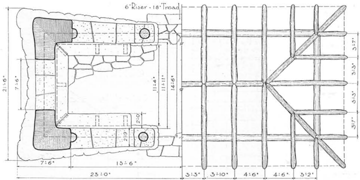
HALF PLAN
