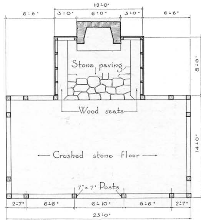
FLOOR PLAN
