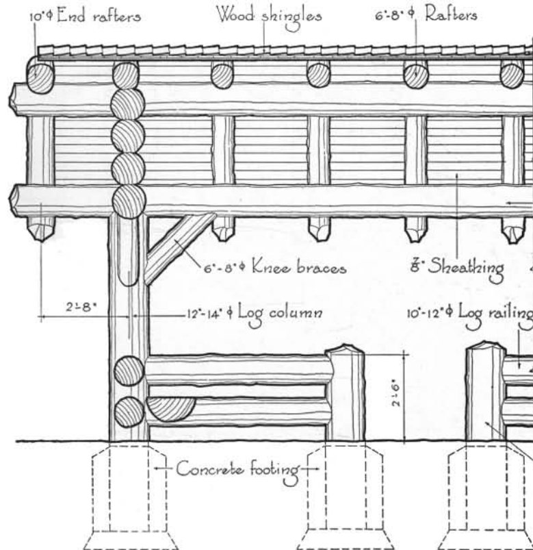
HALF SECTION Scale 7/8" = 1'-0"
