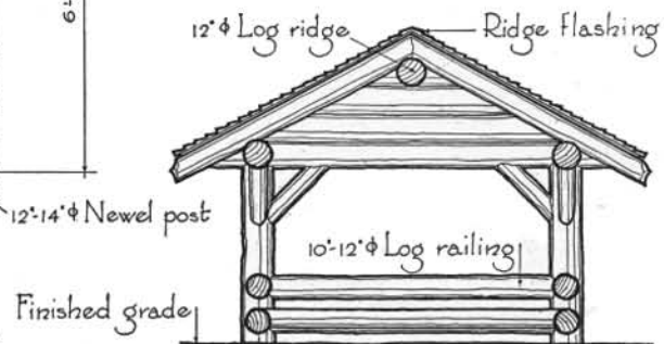
SECTION Scale 5/8" = 1'-0"
