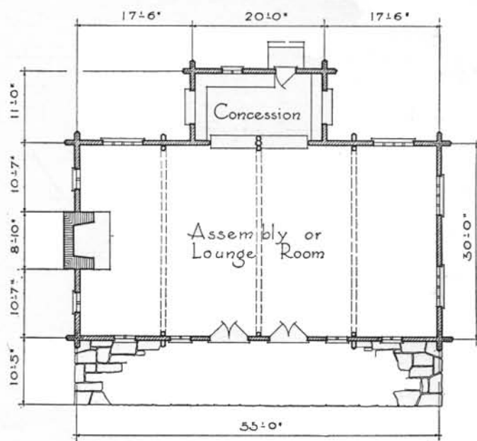
FLOOR-PLAN Scale \frac{1}{8} = 1'-0''
