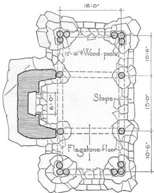
FLOOR PLAN Scale \frac{1}{16} " = 1'-0"
