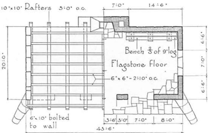
HALF ROOF & FLOOR PLAN
