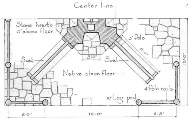
FLOOR PLAN One half only
