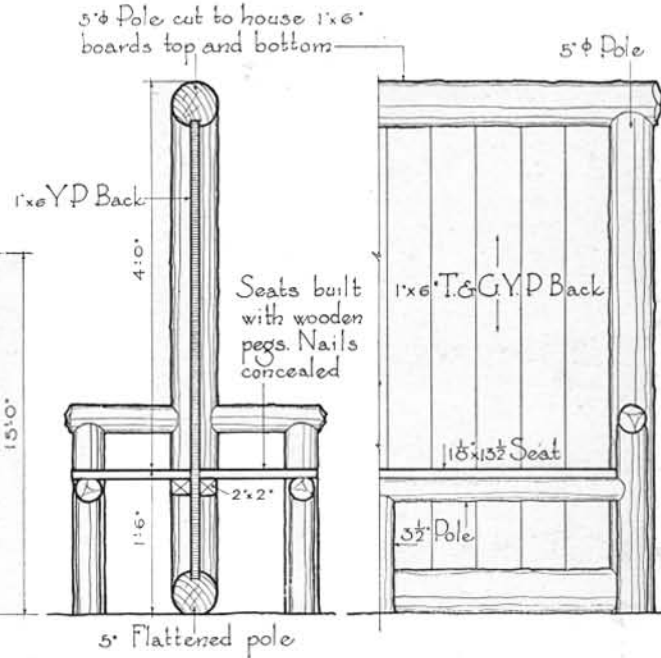
DETAIL OF SEAT Scale \frac{1}{2} " = 1'-0"
