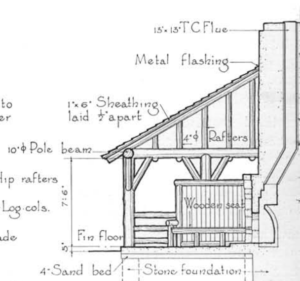
Scale \frac{1}{8} " = 1'-0"
