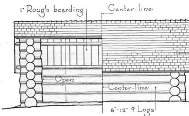
HALF FRONT & REAR ELEVATION
