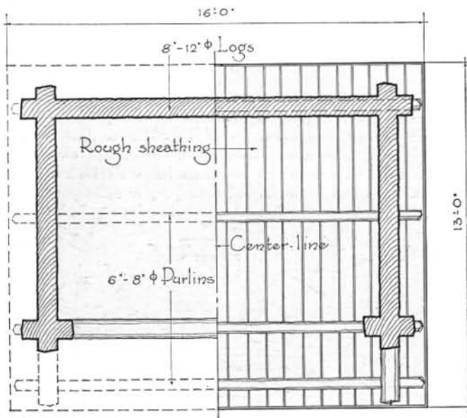
HALF FLOOR- & REFLECTED ROOF PLAN
