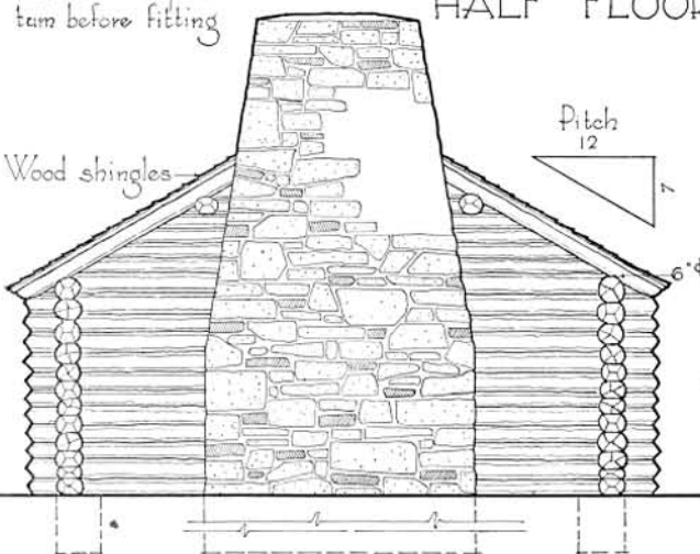
REAR ELEVATION
