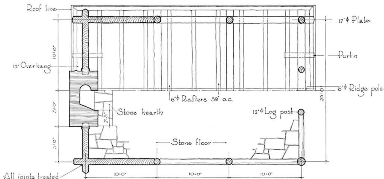
HALF FLOOR & ROOF PLAN
