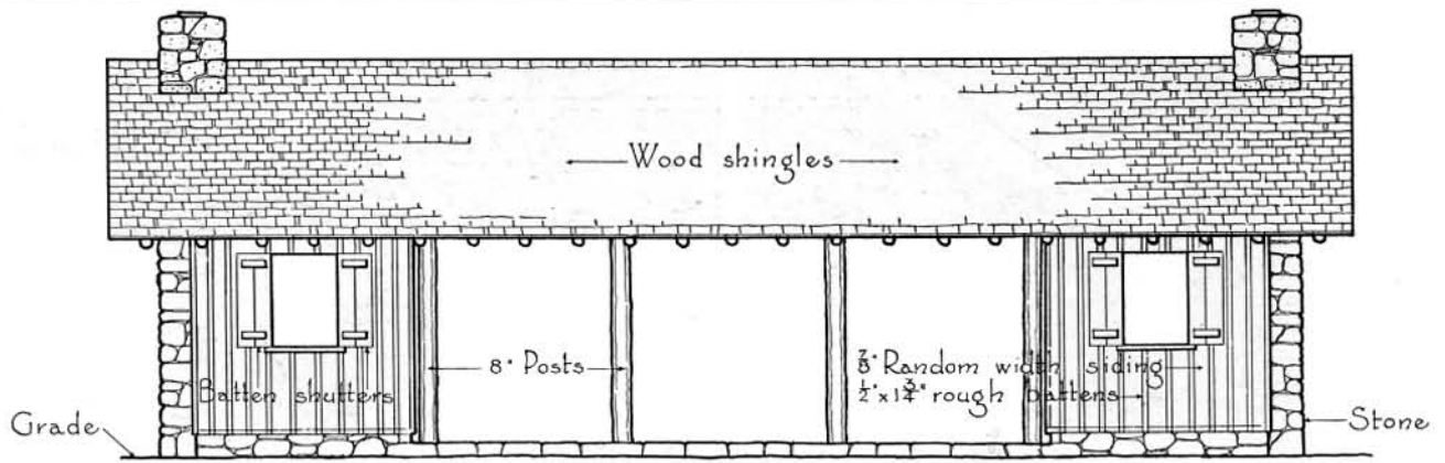
FRONT ELEVATION
