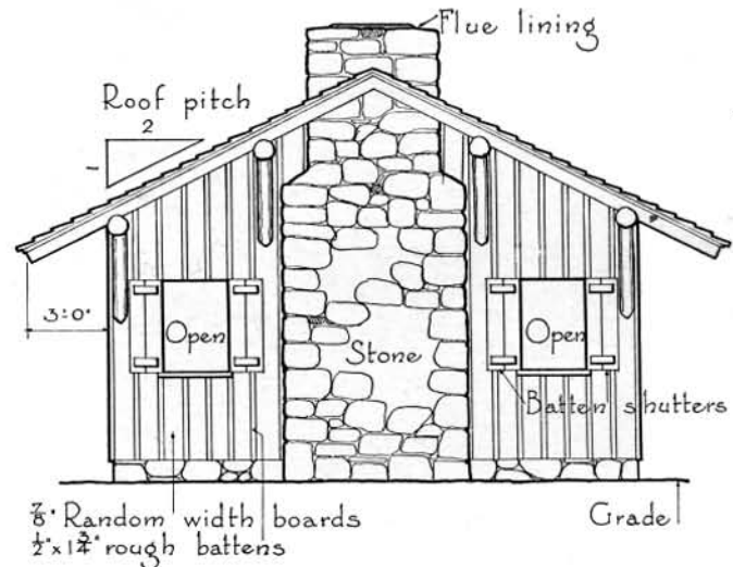
SIDE ELEVATION
