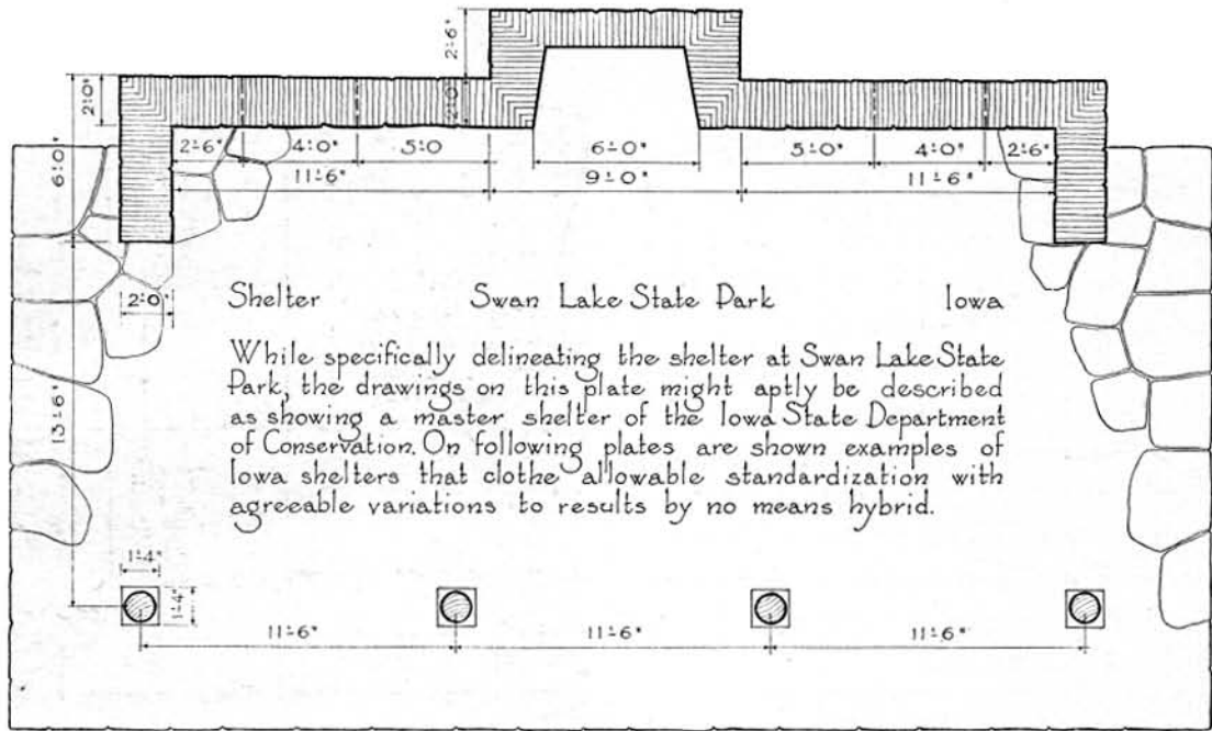
FLOOR PLAN
