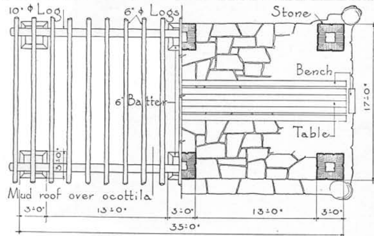
HALF ROOF & FLOOR PLAN Scale \frac{3}{32}'' = 1'-0''
