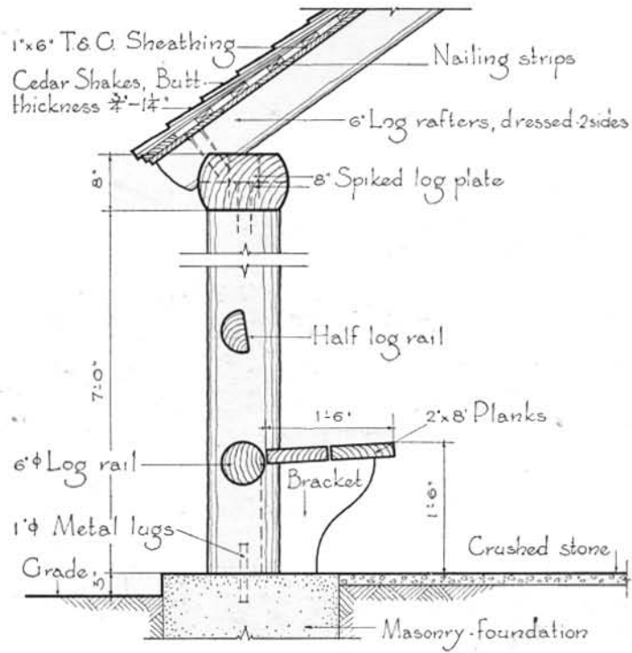
CONSTRUCTION DETAIL
