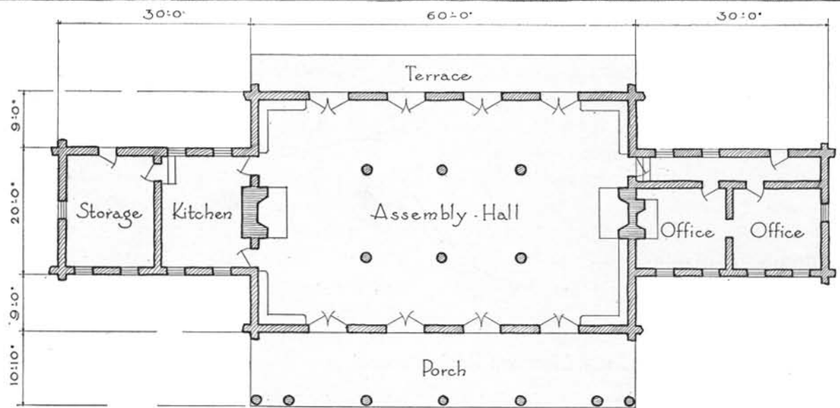
FLOOR-PLAN
