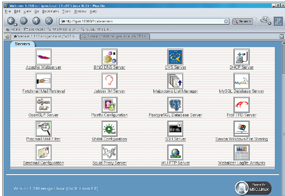
Figure 4-9 Servers administration
