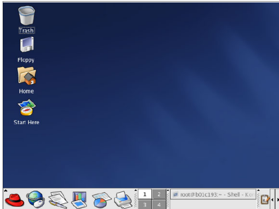
Figure 2-1 KDE desktop
