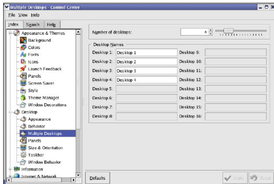
Figure 2-6 Desktops configuration
