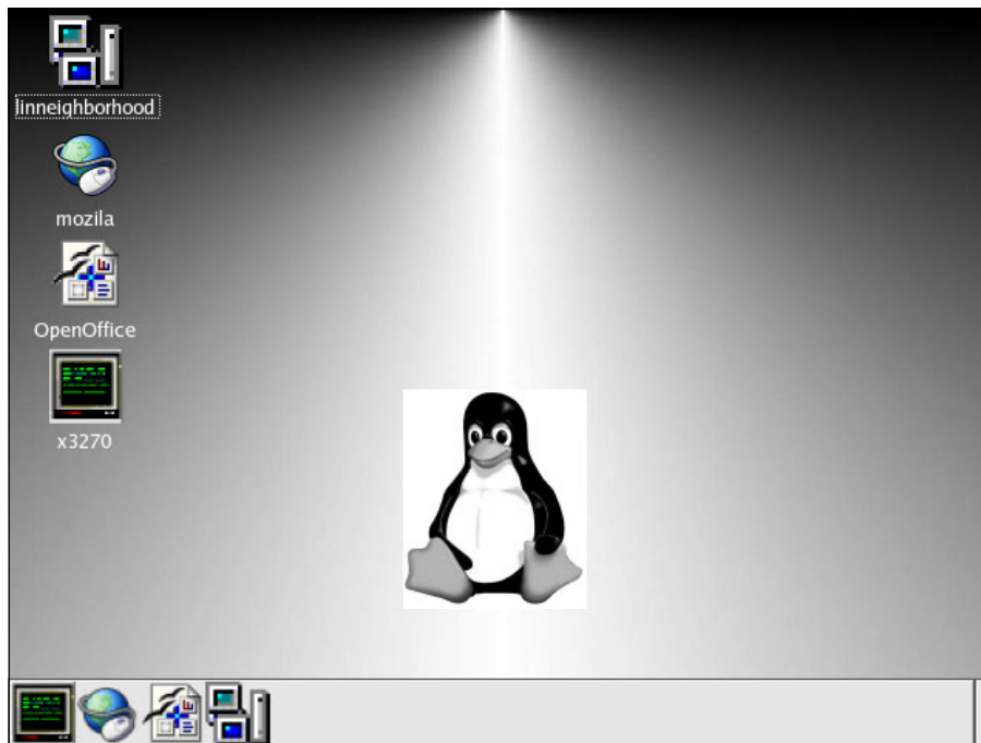
Figure 2-3 Customized desktop
