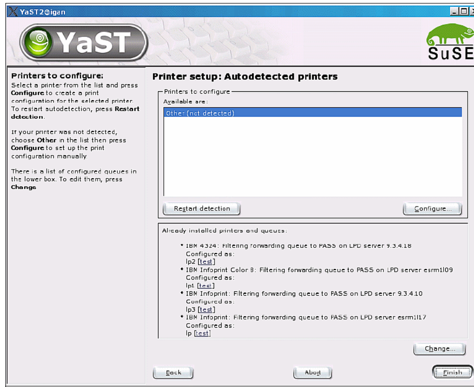
Figure 4-3 Printer setup
