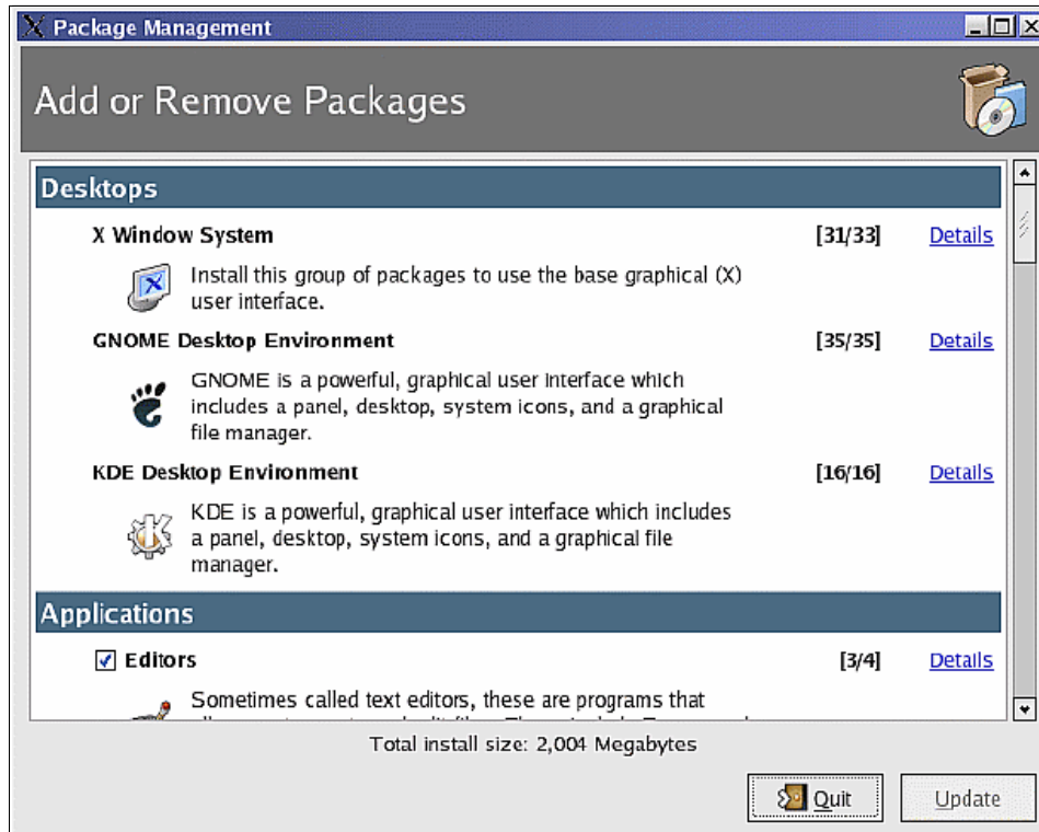
Figure 4-5 Redhat-config-packages
