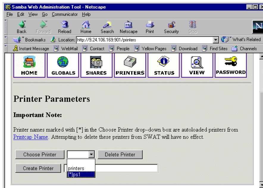
Figure 39. Selecting a printer
