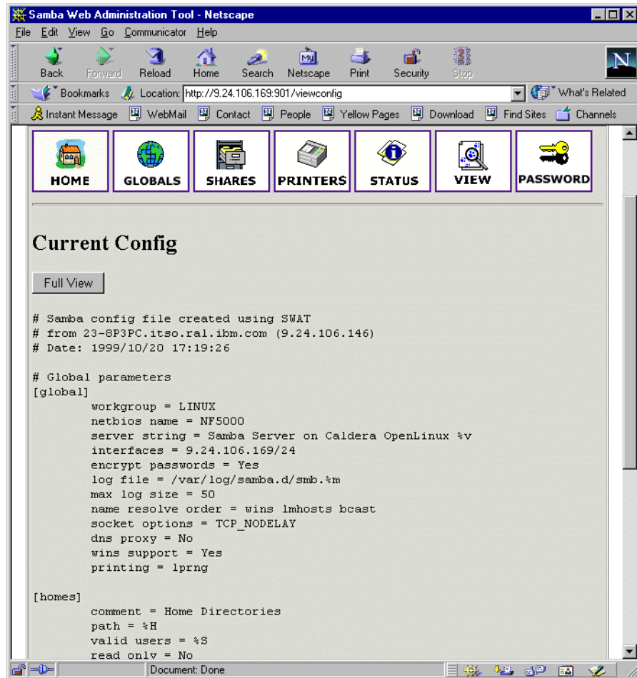
Figure 42. View section of SWAT
