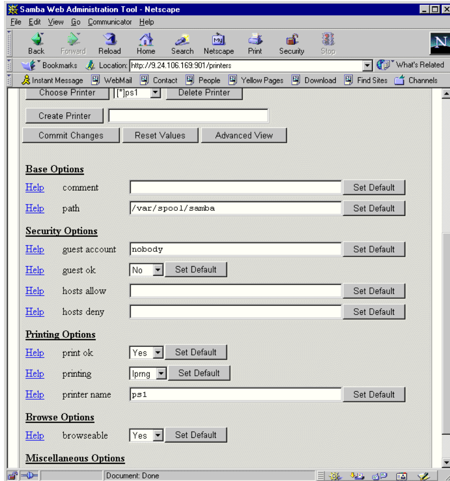
Figure 58. Printer properties
