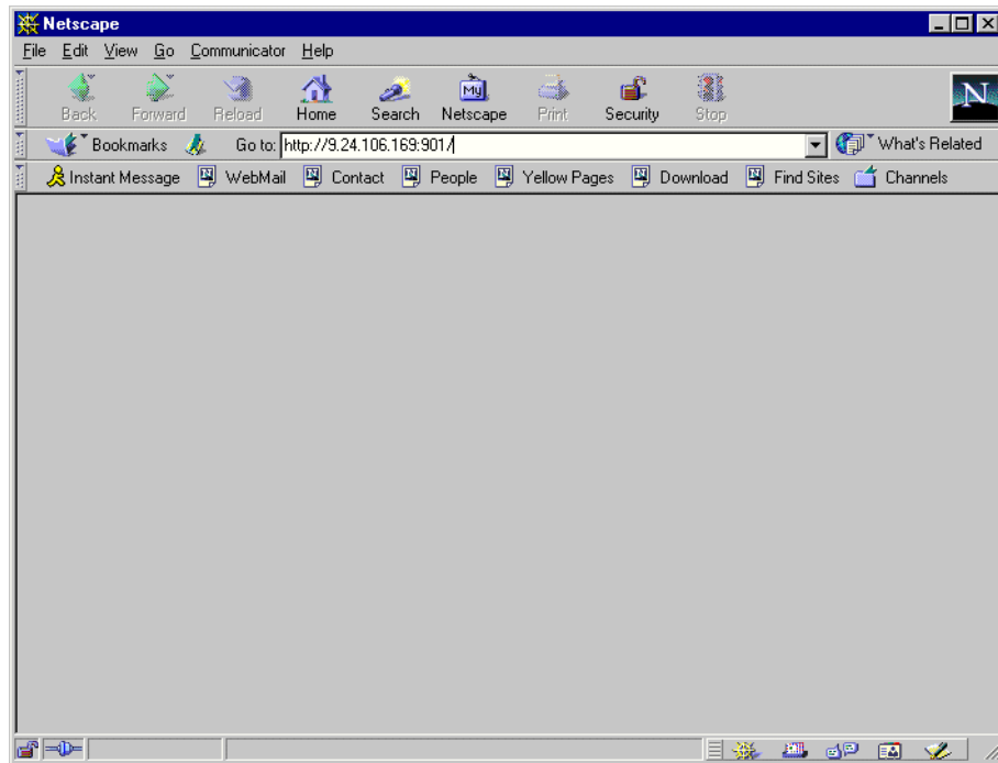
Figure 44. Starting SWAT
