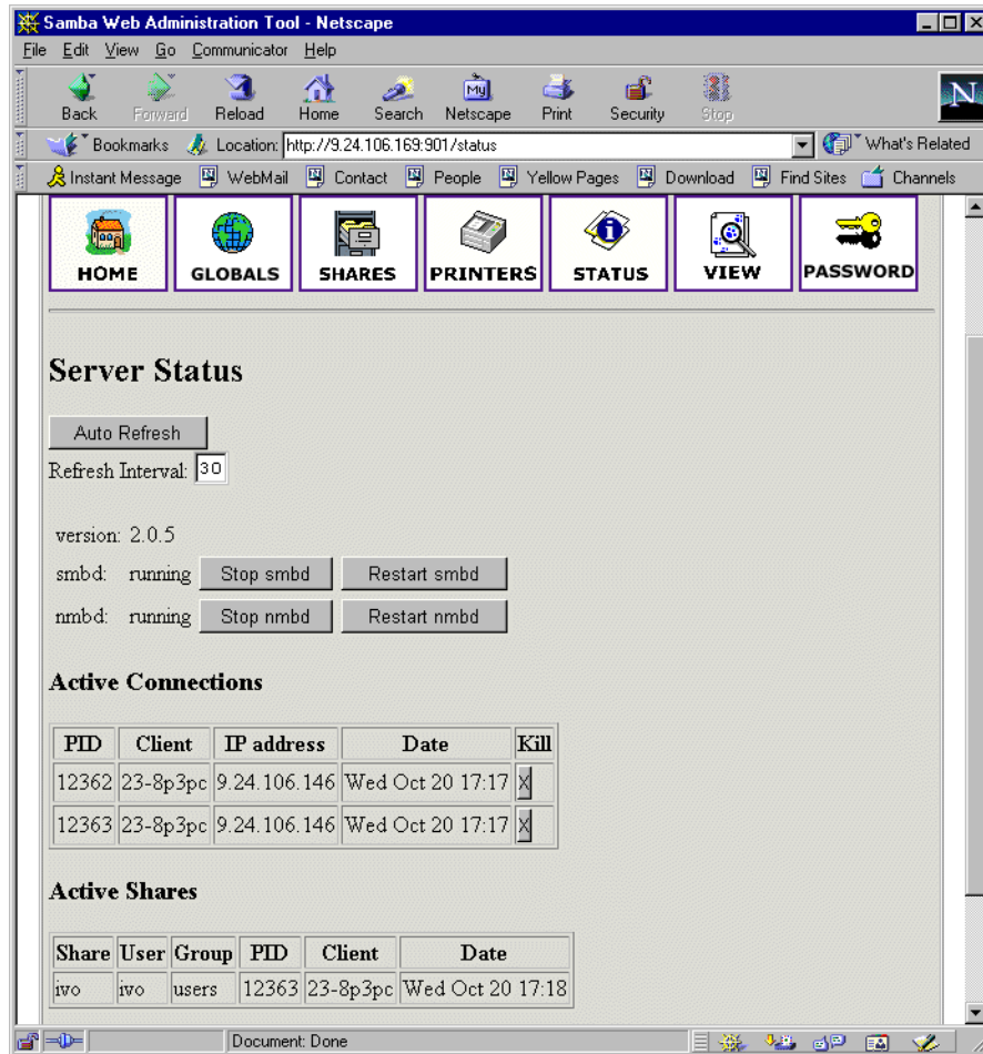
Figure 90. Status section
