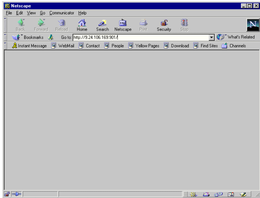
Figure 2. Starting SWAT
