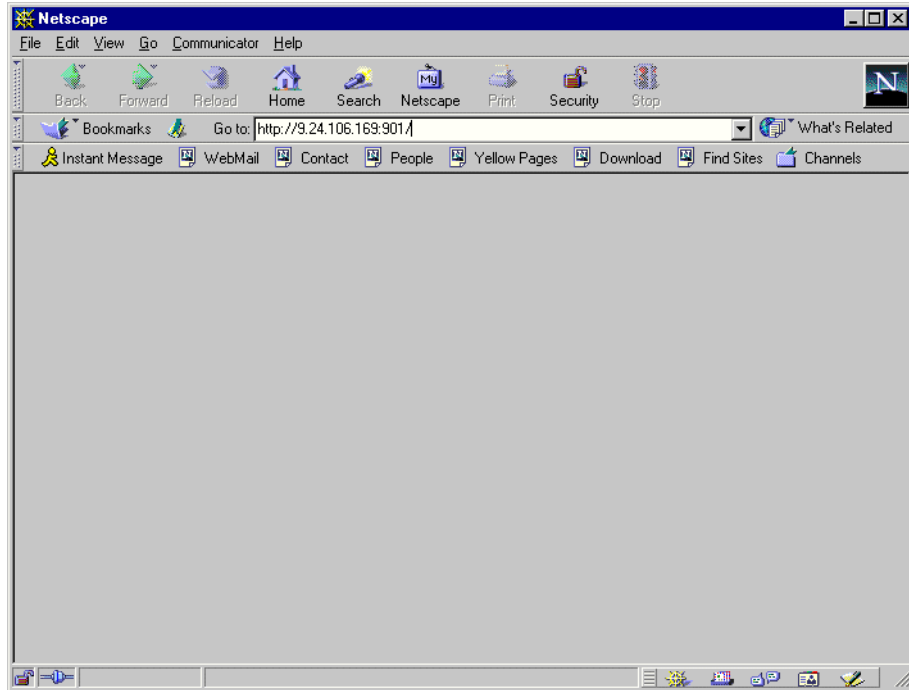
Figure 75. Starting SWAT
