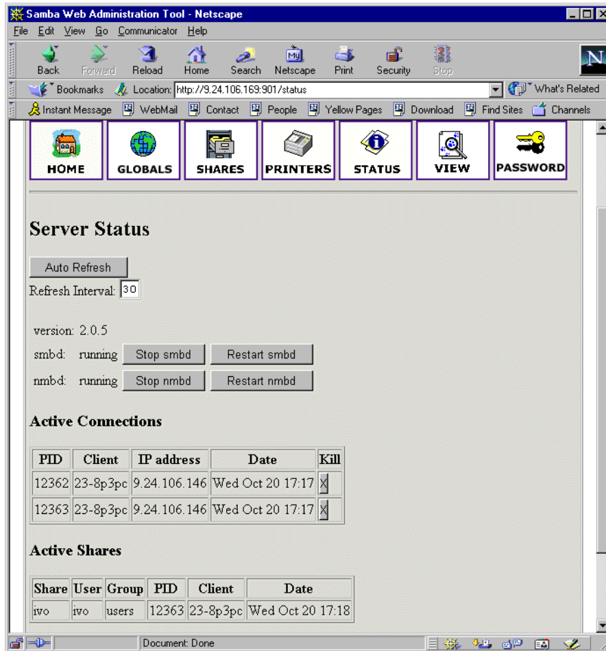
Figure 41. Status section
