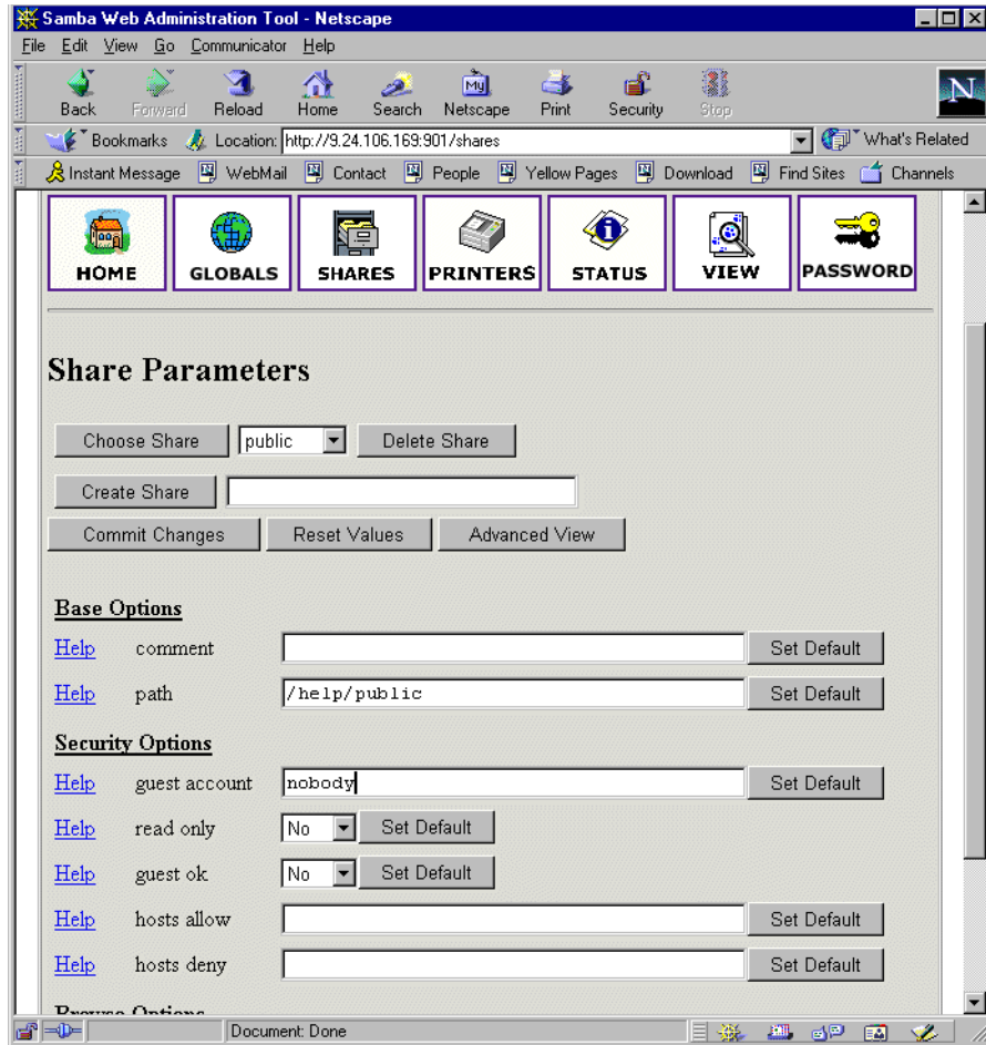
Figure 84. Entering the new share parameters
