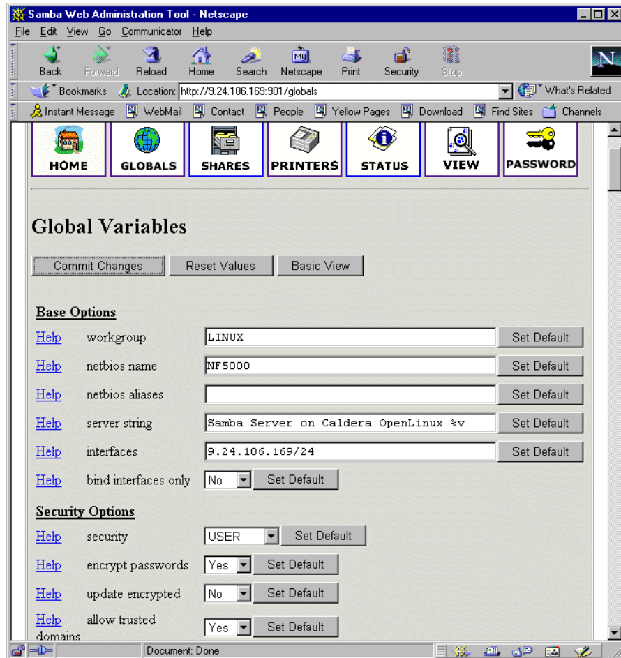
Figure 5. Global section in SWAT
