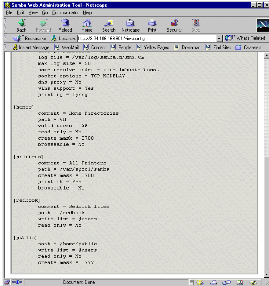
Figure 36. Viewing the smb.conf configuration file
