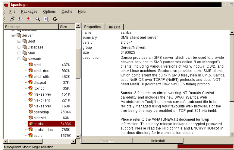
Figure 21. Checking for the Samba package
