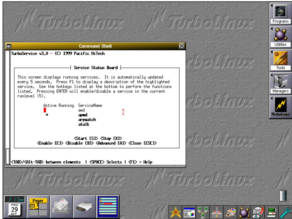
Figure 72. turboservice Service status board
