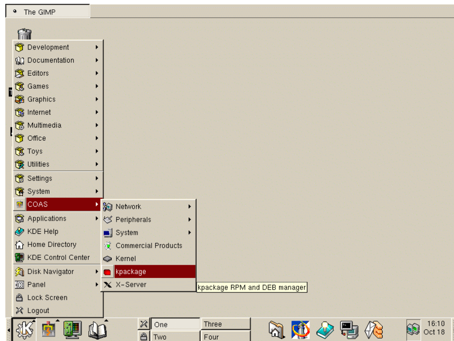
Figure 20. Starting kpackage
