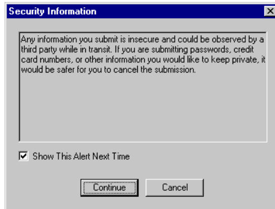
Figure 6. Security warning
