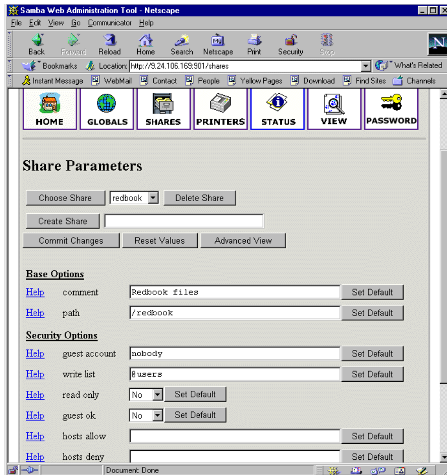
Figure 51. Share properties
