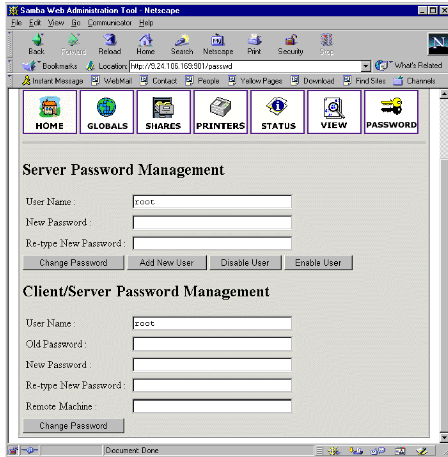
Figure 92. Managing passwords
