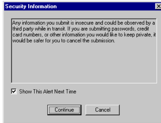
Figure 48. Security warning
