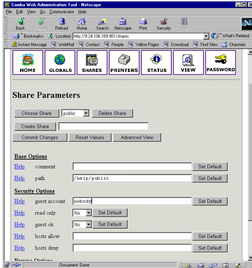
Figure 53. Entering the new share parameters
