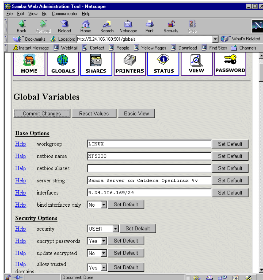
Figure 47. Global section in SWAT
