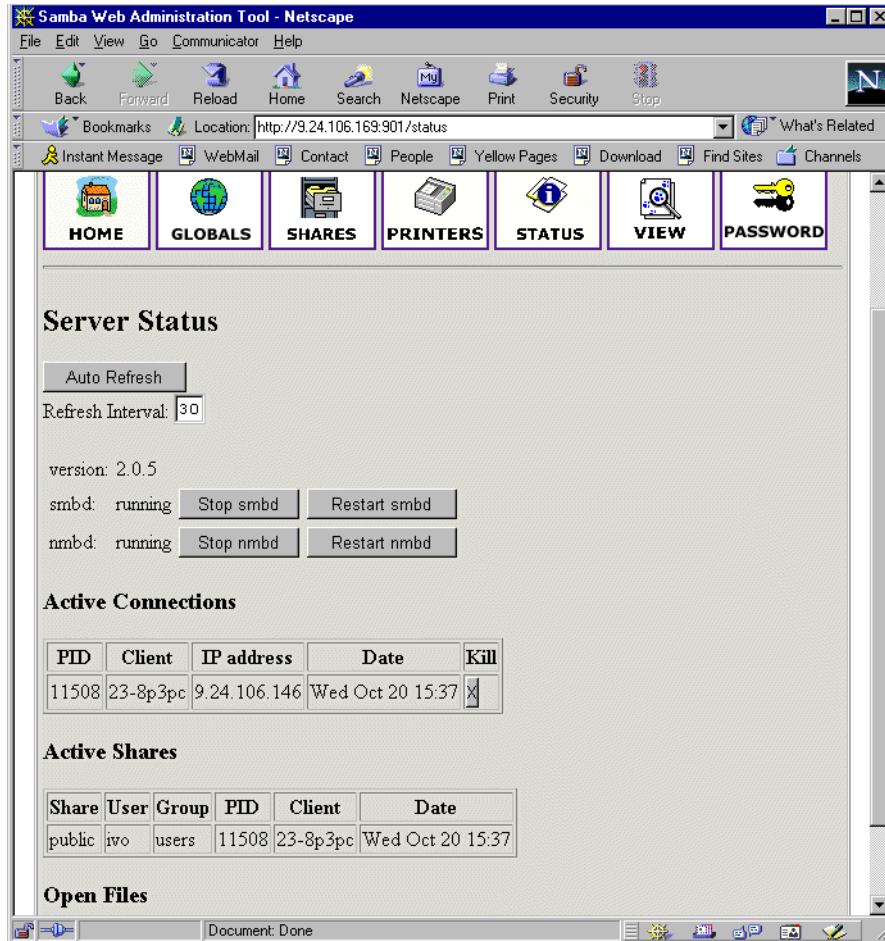
Figure 55. Restarting the Samba server
