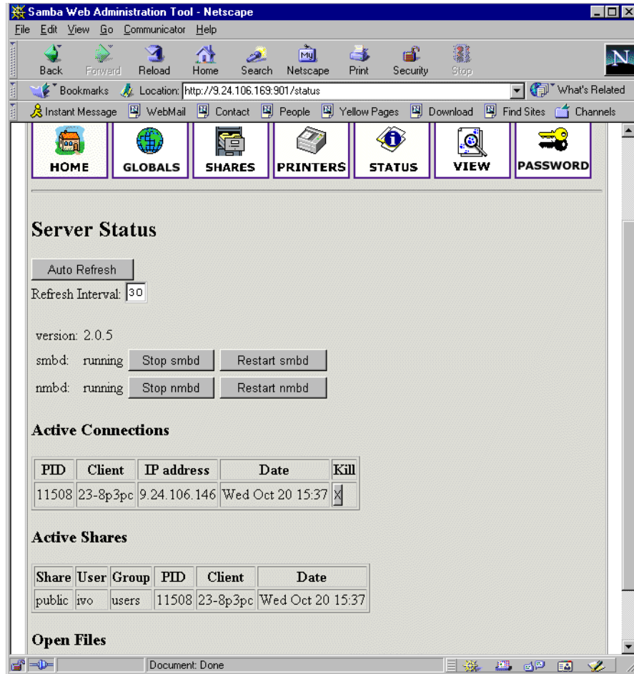
Figure 86. Restarting the Samba server
