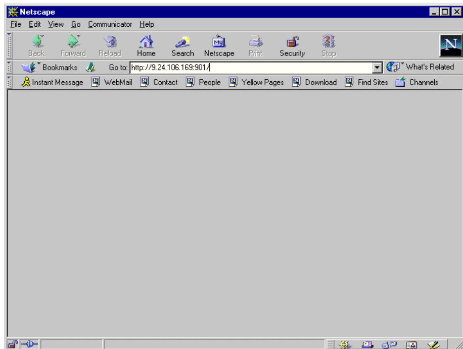
Figure 26. Starting SWAT
