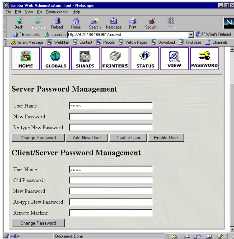
Figure 43. Managing passwords
