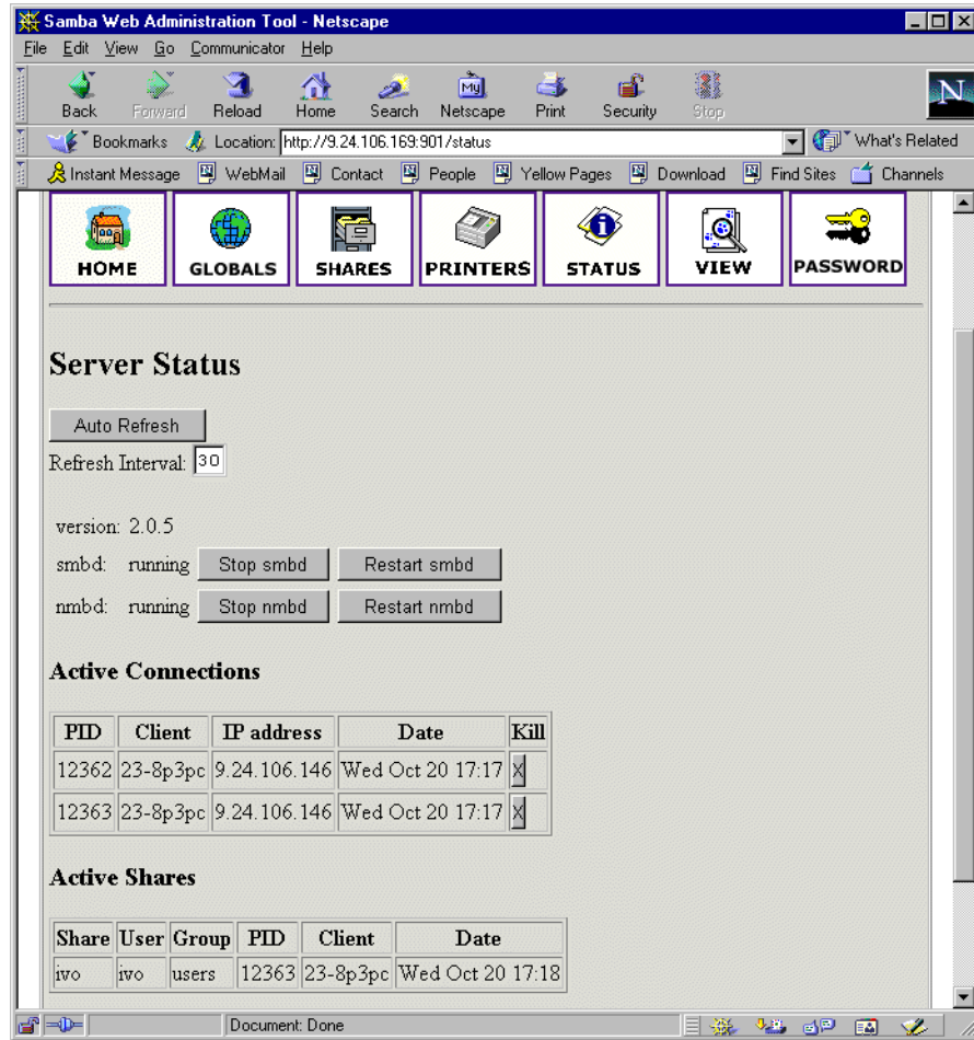
Figure 59. Status section
