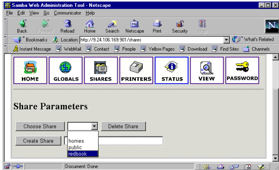
Figure 32. Choosing a share to view
