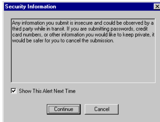
Figure 79. Security warning
