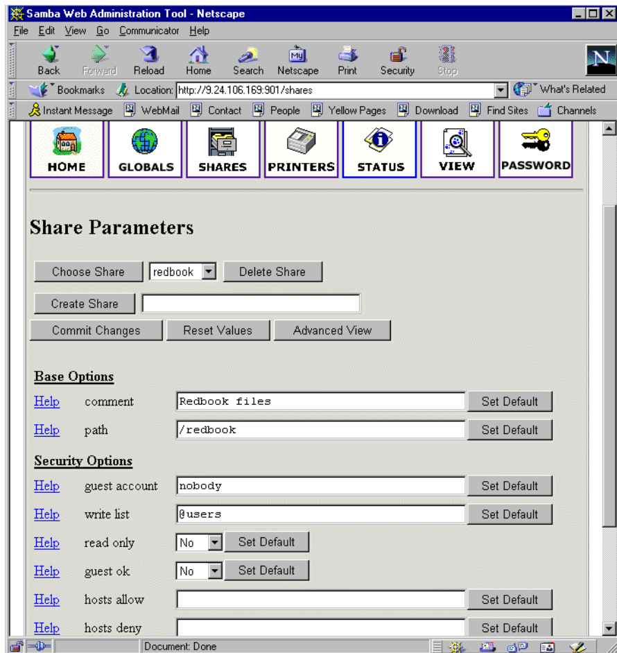
Figure 33. Share properties
