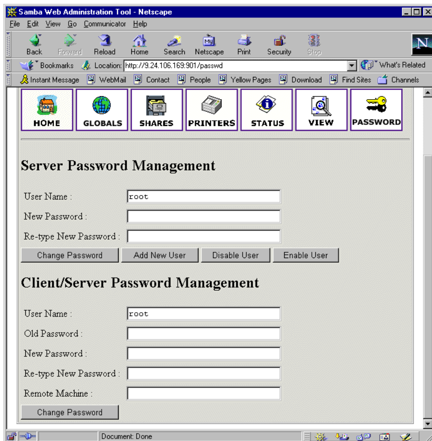
Figure 61. Managing passwords
