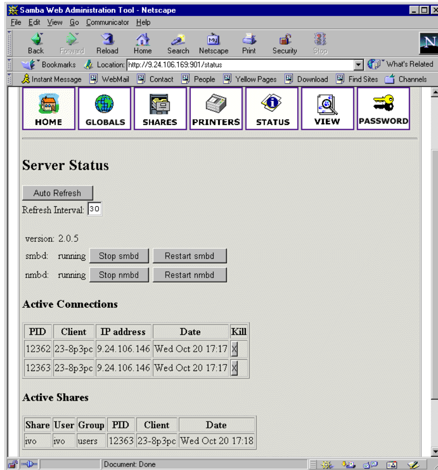
Figure 17. Status section
