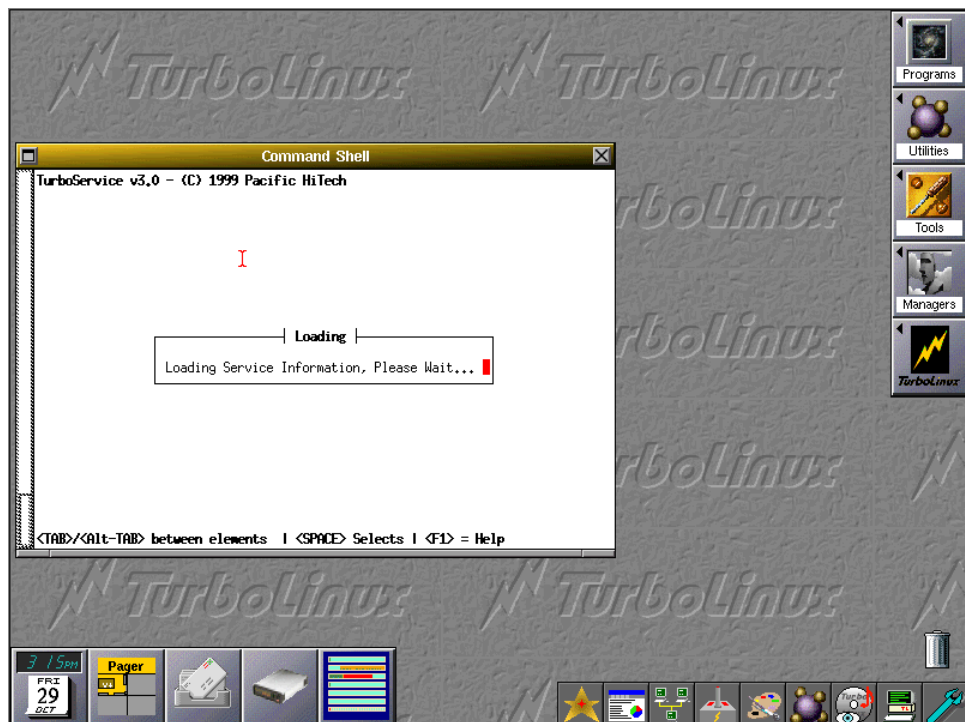
Figure 71. Starting turboservice
