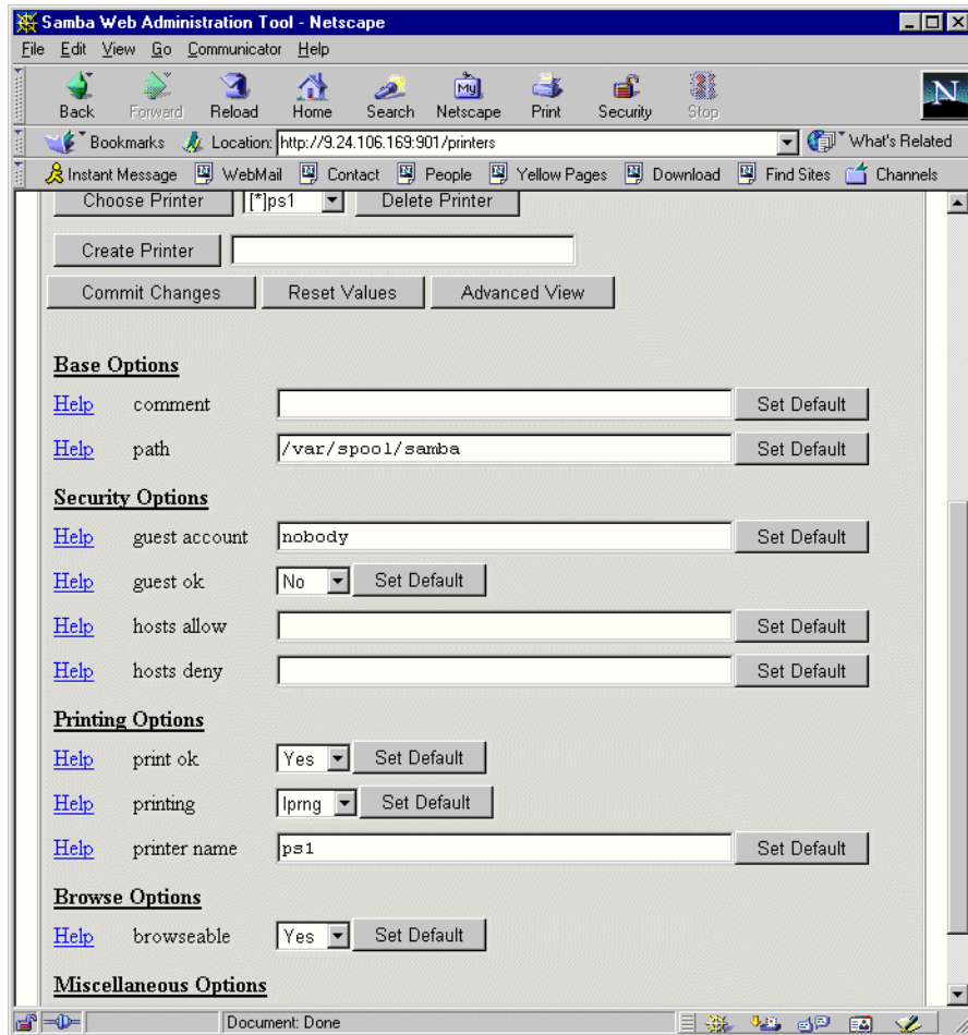
Figure 89. Printer properties
