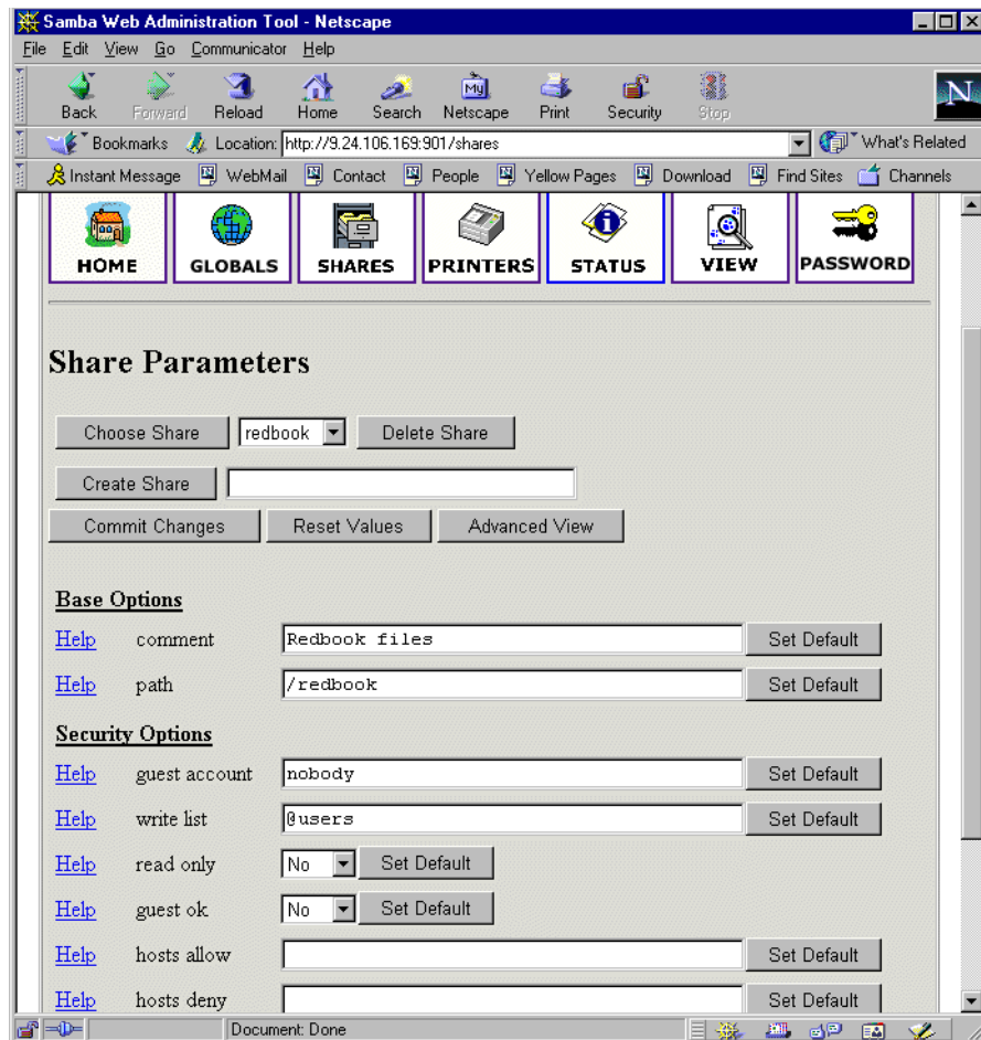
Figure 82. Share properties
