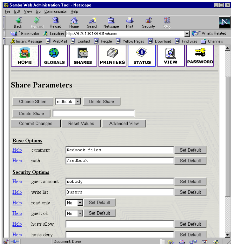
Figure 9. Share properties
