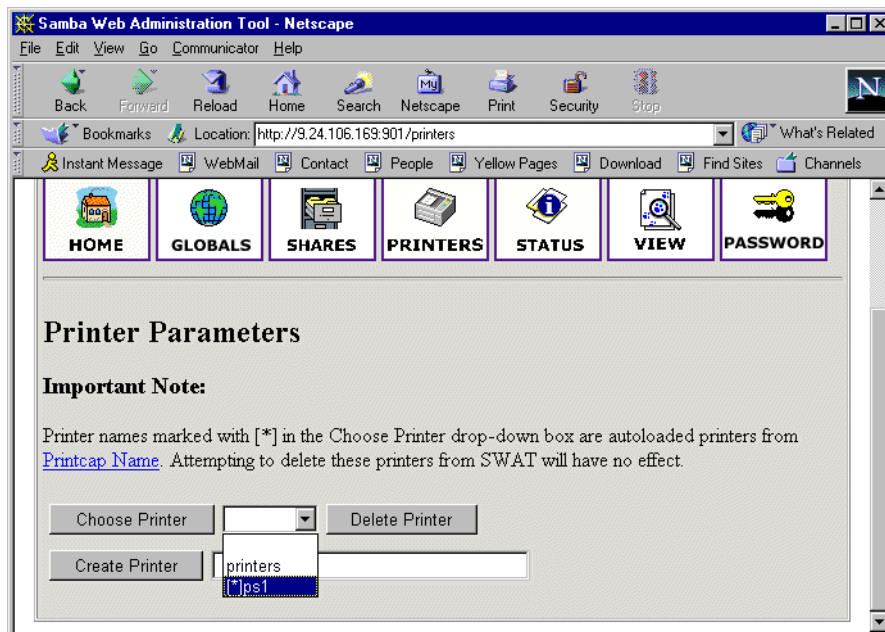
Figure 15. Selecting printer
