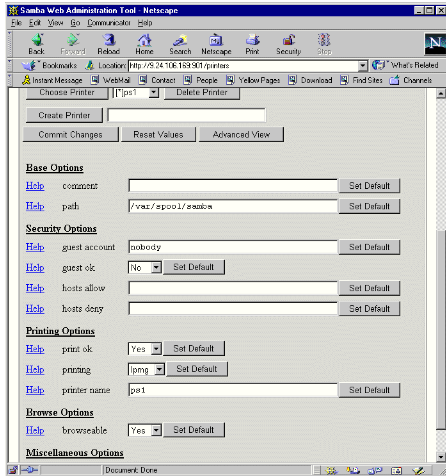
Figure 16. Printer properties
