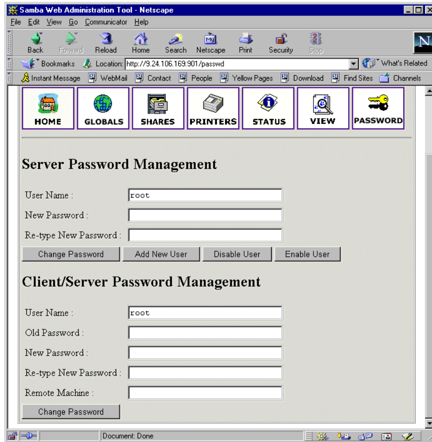
Figure 19. Managing passwords
