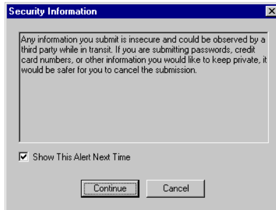
Figure 30. Security warning
