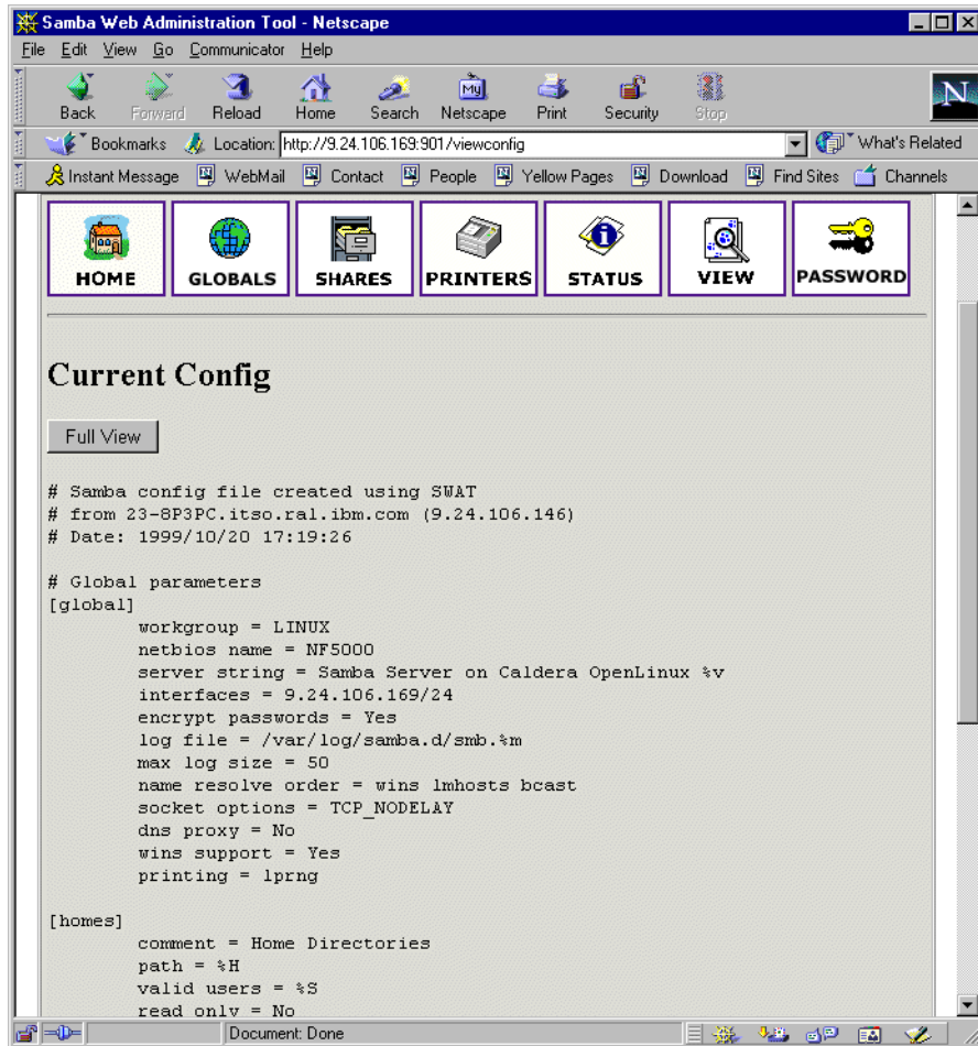
Figure 18. View section of SWAT
