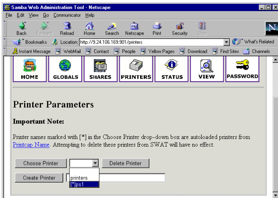
Figure 88. Selecting a printer
