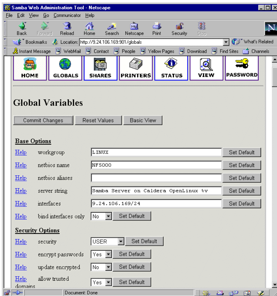
Figure 78. Global section in SWAT
