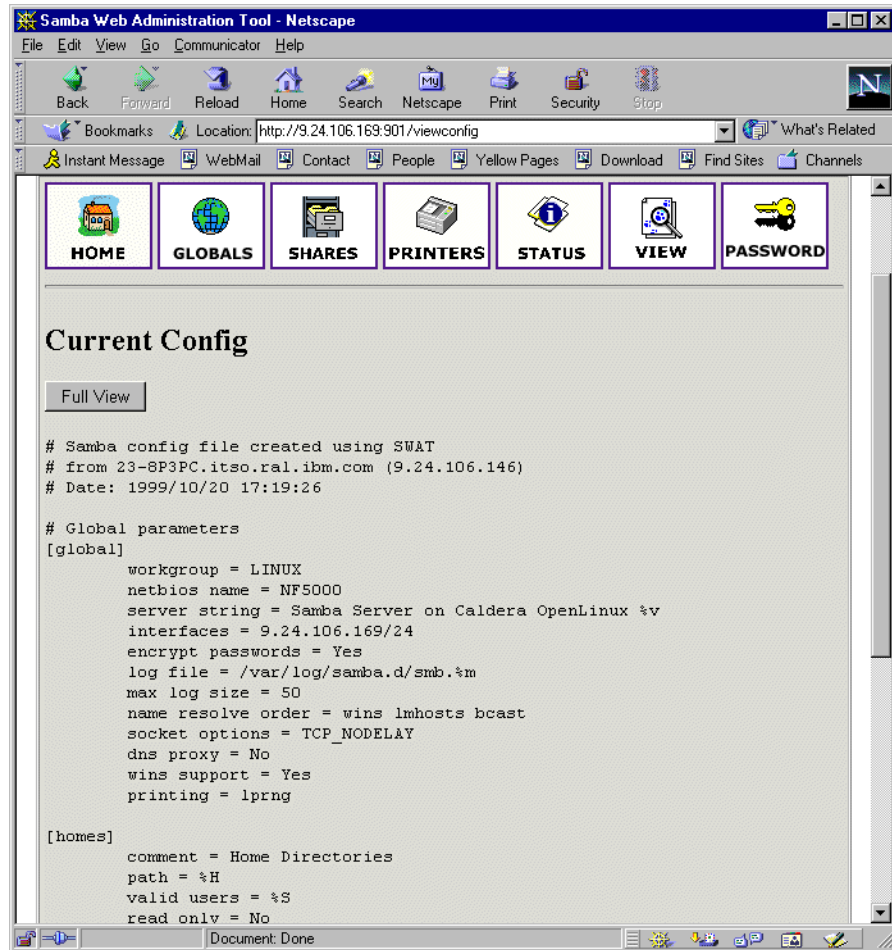
Figure 91. View section of SWAT
