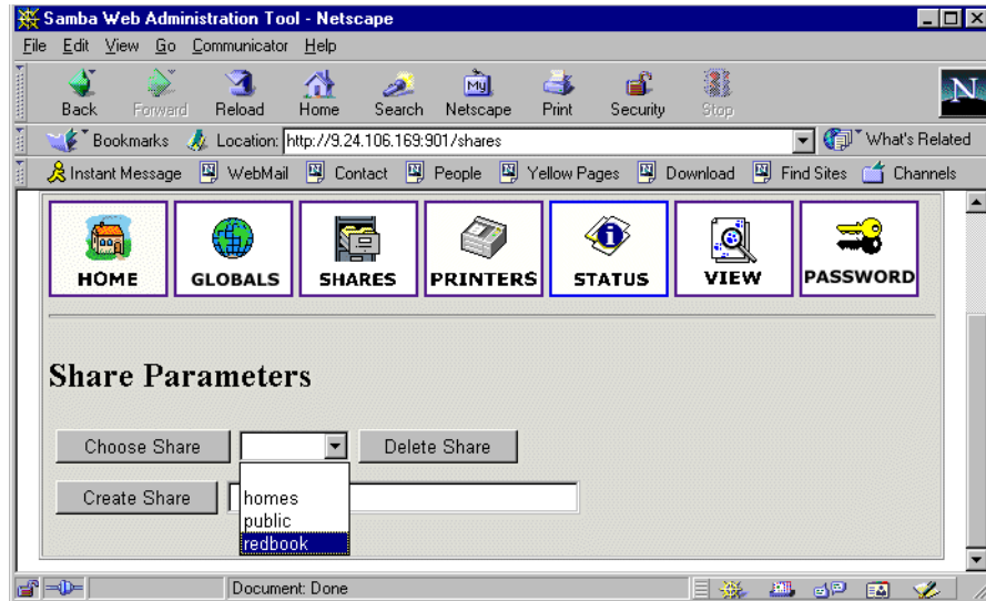
Figure 81. Choosing a share to view
