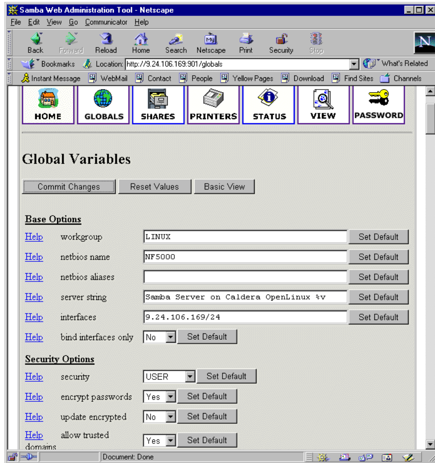
Figure 29. Global section in SWAT
