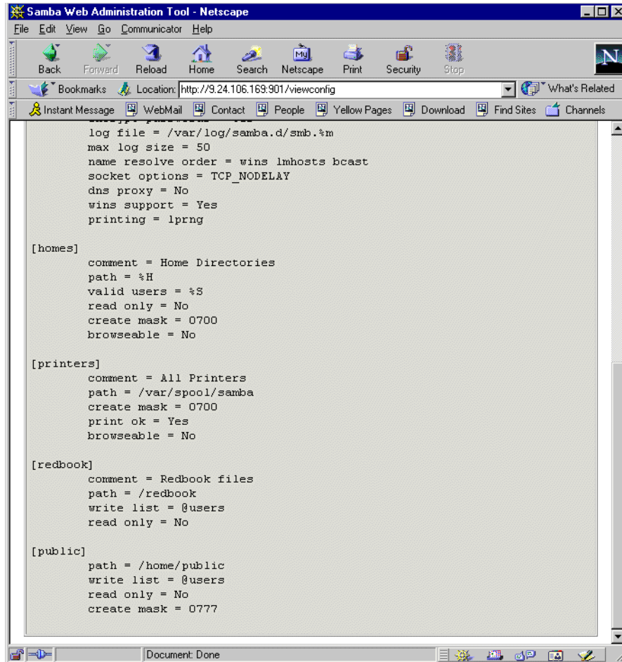
Figure 85. Viewing the smb.conf configuration file
