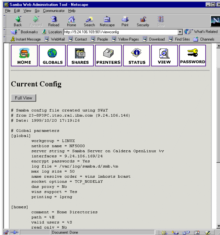
Figure 60. View section of SWAT
