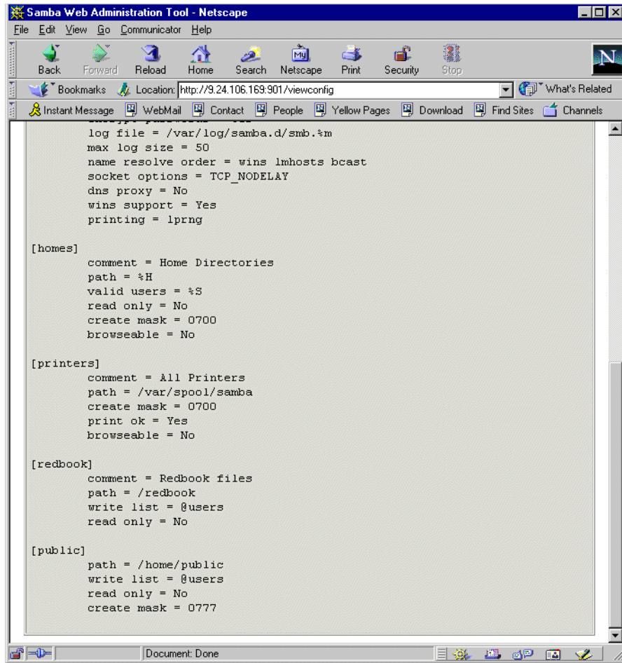
Figure 54. Viewing the smb.conf configuration file
