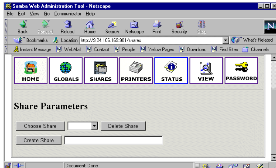
Figure 31. Shares section in SWAT
