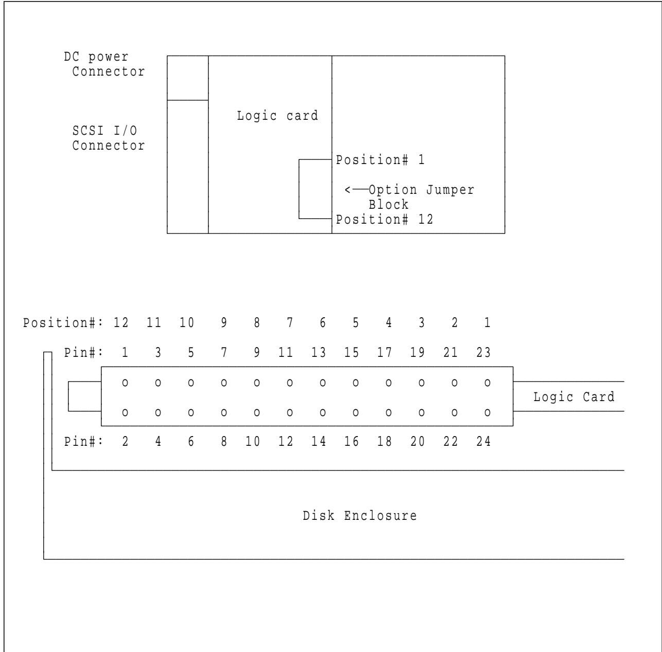
Figure 17. Jumper Pins
