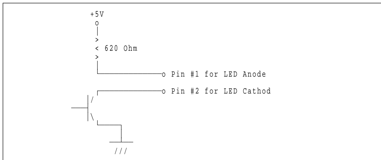
Figure 21. LED Circuit
