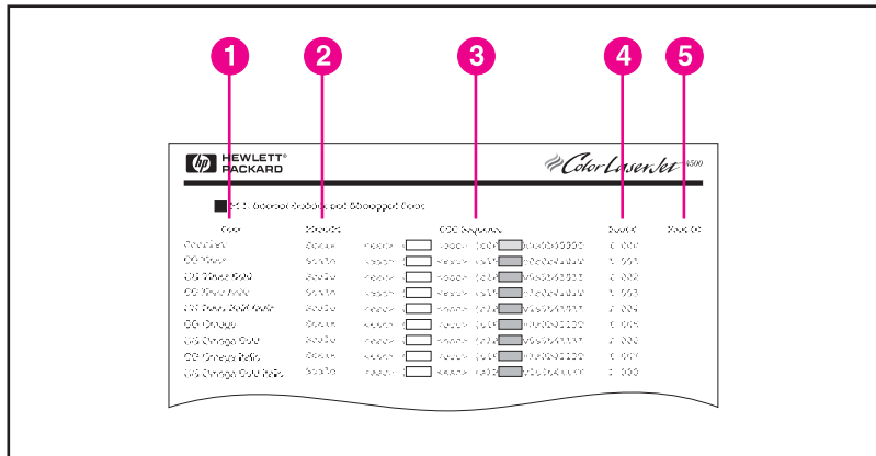
Figure 5-1 Font List
