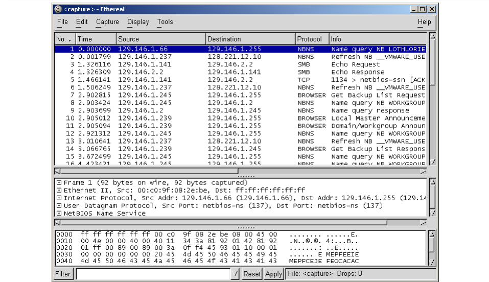
Figure 39.2 Main Ethereal Data Window.
