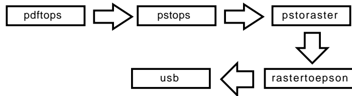
Figure 22.12 PDF to USB Chain.
