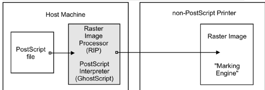
Figure 22.3 Ghostscript as a RIP for Non-PostScript Printers.
