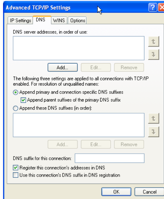
Figure 8.4 DNS Configuration.
