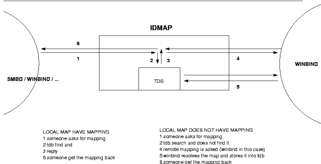
Figure 24.1 Winbind Idmap
