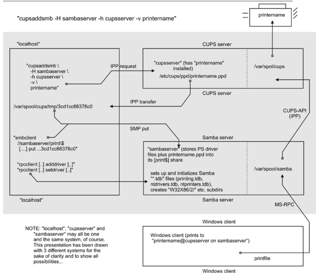
Figure 22.16 cupsaddsmb Flowchart.
