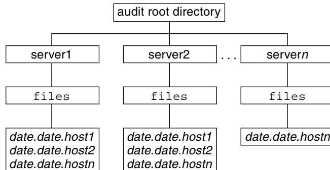
FIGURE 31-1 Audit Trail Storage Sorted by Host
