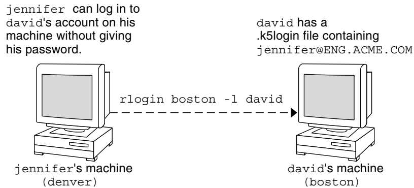
FIGURE 26-1 Using the .k5login File to Grant Access to Your Account
