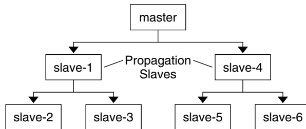
FIGURE 8-2 Example of Parallel Propagation Configuration
