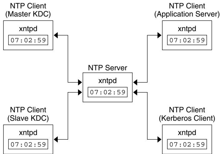
FIGURE 8-1 Synchronizing Clocks by Using NTP
