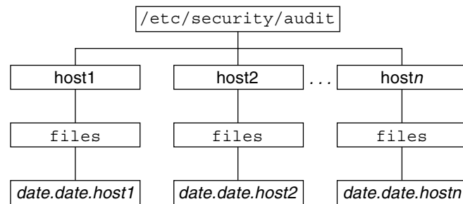
FIGURE 25–1 Audit Trail Storage Sorted by Host
