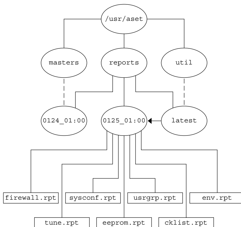
FIGURE 20-1 Structure of the ASET reports Directory
