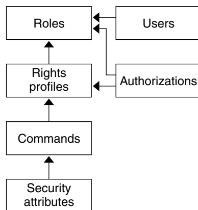
FIGURE 17-1 Solaris RBAC Element Relationships
