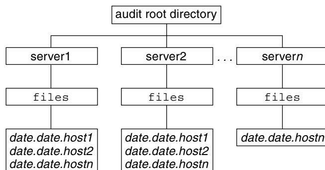
FIGURE 25-2 Audit Trail Storage Sorted by Server
