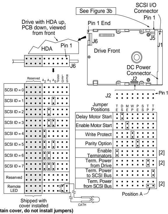
Figure 3a. Drive configurator, Hawk 2LP family N/ND models
