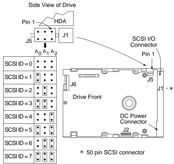
Figure 3b. Drive configurator, Hawk 2LP family N/ND models
