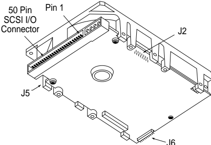
Figure 2. Hawk 2LP family N/ND model drives I/O connection (50 pin SCSI I/O connector). "N" model drive terminators (not visible) are not removable.
