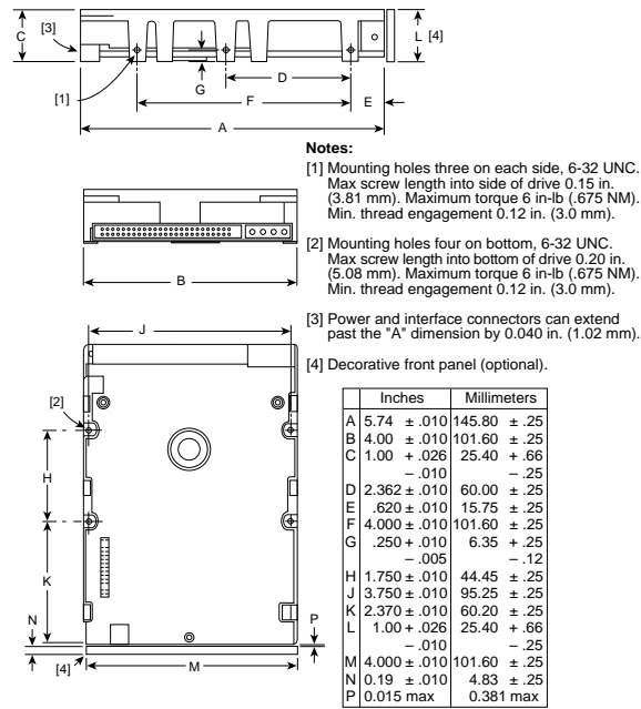
Figure 4. Hawk 2LP family N/ND model mounting dimensions (50 pin SCSI I/O connector)
