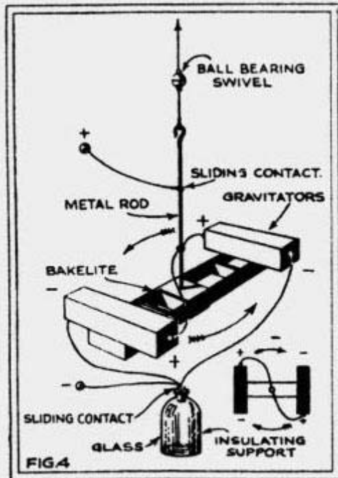
FIG 4 A GRAVITATOR ROTOR IS SIMPLY AN ASSEMBLY OF UNITS SO MADE THAT ROTATION RESULTS UNTIL THE IMPULSE IS EXHAUSTED.
