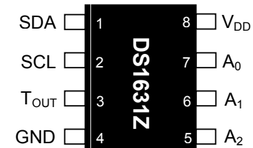
DS1631Z—8-pin SO (150mil)
