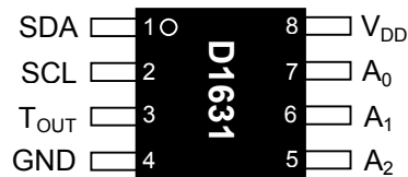
DS1631U— \mu SOP
