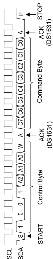
a) Issue a "Start Convert T" or "Stop Convert T" Command
