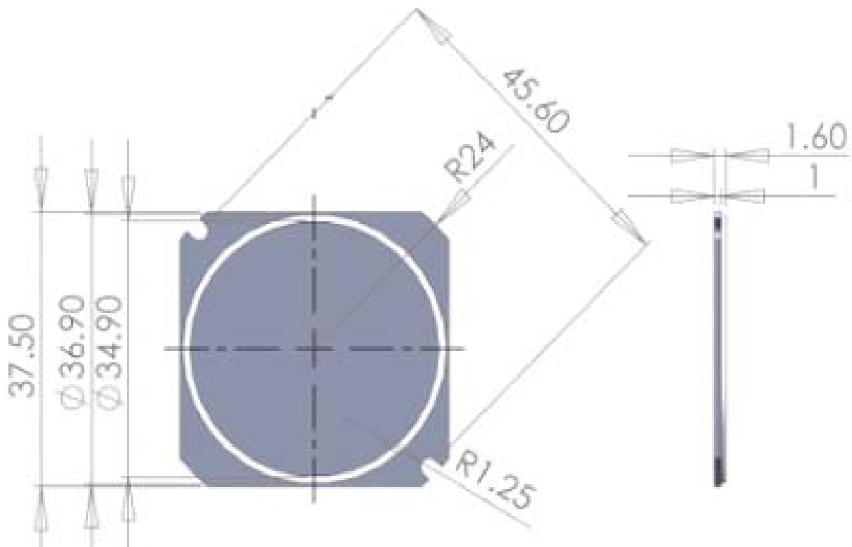
LCOB50-20W030XXFR60
