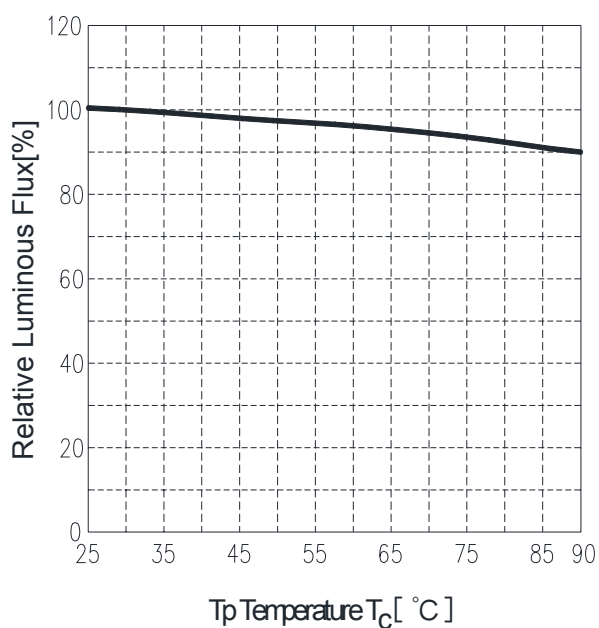
Relative Luminous Flux (@640mA) vs. T_p Temperature
