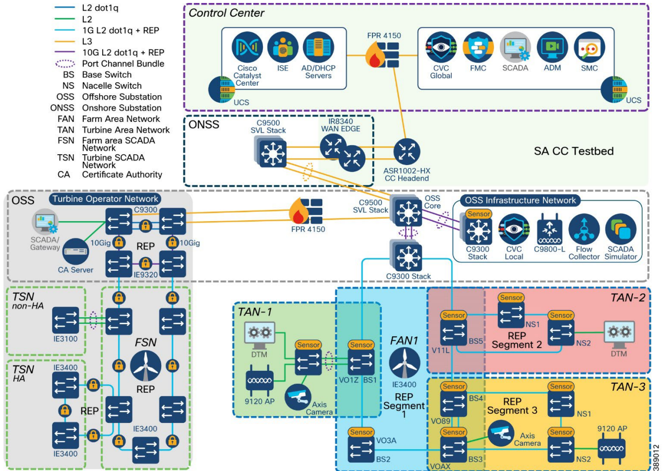
Figure 2-1: Wind Farm 1.1 Wired Network Topology
