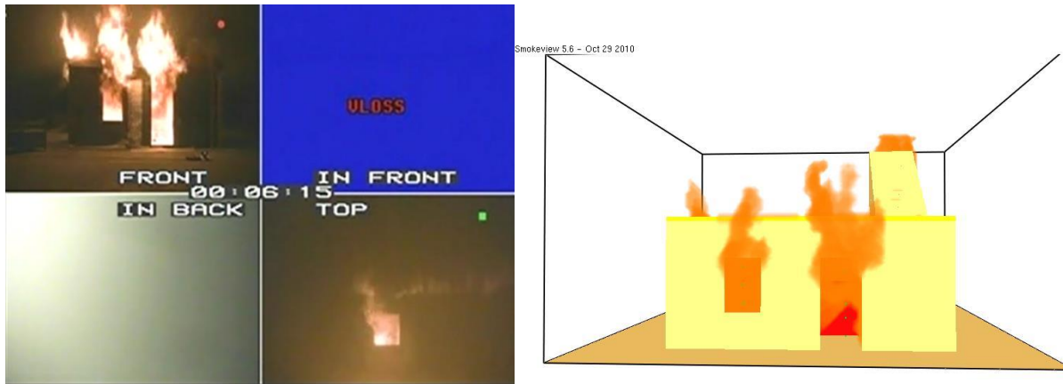
Figure 22 Comparison of flames towards end of test
