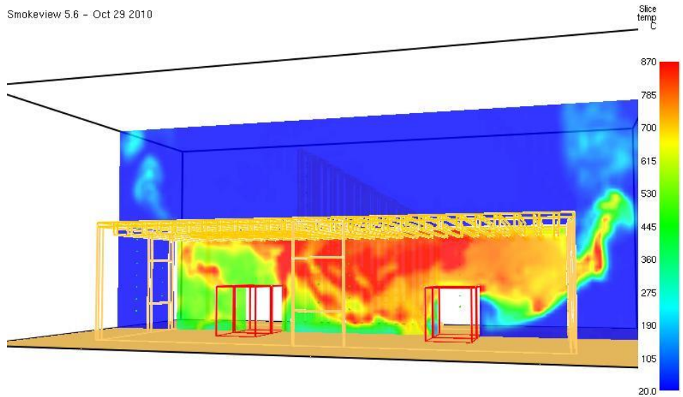
Figure 31 Temperature contour at 300 s
