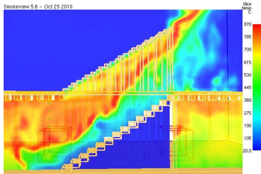
Figure 32 Gas temperature contours within stairway (in a plane though the middle)
