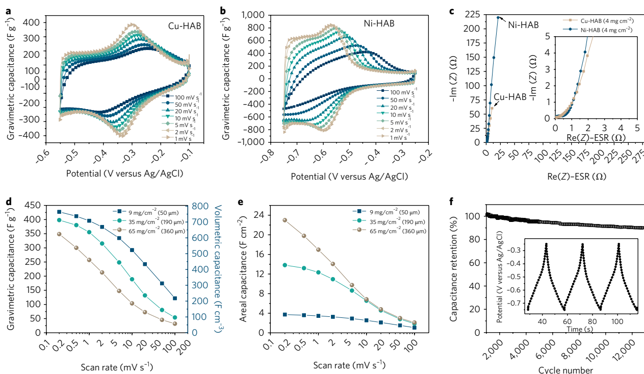
Fig. 3 | Electrochemical performance of HAB MOFs in 1M KOH. a, b , Cyclic voltammetry profiles collected at different scan rates for Cu-HAB ( a ) and Ni-HAB ( b ) electrodes. c , EIS data collected for Cu-HAB Ni-HAB electrodes with weight loadings of 4 \text{ mg cm}^{-2} . Inset: enlargement of high-frequency regions. \text{Re}(Z) -ESR represents the real part of the system impedance, in which the equivalent series resistance (ESR) was subtracted, and \text{Im}(Z) stands for the imaginary part of the system impedance. ESR, equivalent series resistance. d , Gravimetric and volumetric rate performance for Ni-HAB pellet electrodes with different areal densities of 9, 35 and 65 \text{ mg cm}^{-2} . e , Areal rate performance for the Ni-HAB electrodes with different weight loadings. f , Capacitance retention data collected by galvanostatic charge discharge at 10 \text{ A g}^{-1} . Inset: galvanostatic charge-discharge profiles.
