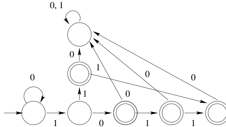
FIG. 5.1. Automaton accepting the base-2 representations of the primes p where 2 \leq p \leq 11
