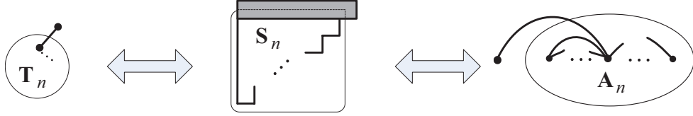
Figure 10: Construction of \mathbf{X}_{n+1} using f_L .
