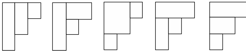
Figure 5: Staircase tilings \mathbf{S}_3 .
