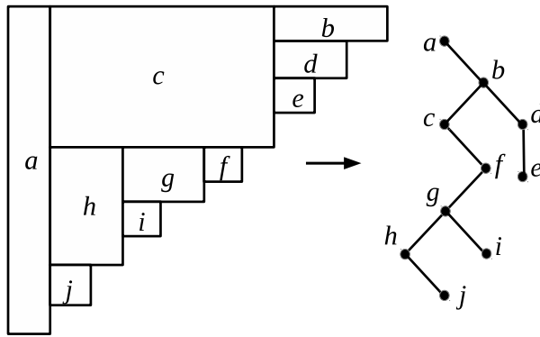
Figure 28: A full example for the case n = 10 ( \beta^{-1} : \mathbf{S}_n \rightarrow \mathbf{T}_n ).
