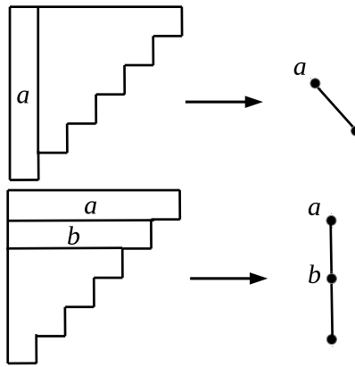
Figure 24: A full example for the case n = 10 ( \beta : \mathbf{T}_n \rightarrow \mathbf{S}_n ).
