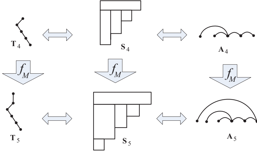
Figure 9: Examples of the construction of \mathbf{X}_{n+1} using f_M .
