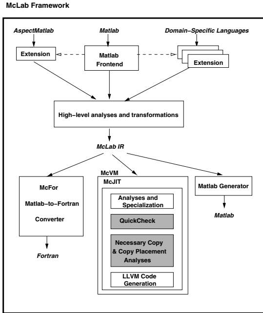
Fig. 1. Overview of McLab (shaded boxes correspond to analyses in this paper)
