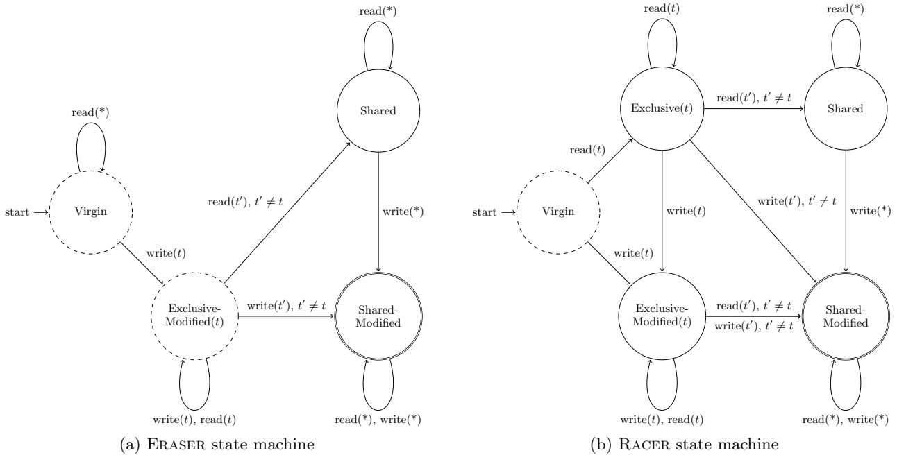
Figure 8: ERASER and RACER state machines; dashed states do no lock refinement; double-lined states report race potential
