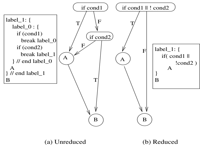
Figure 5. Reducing using the || operator
