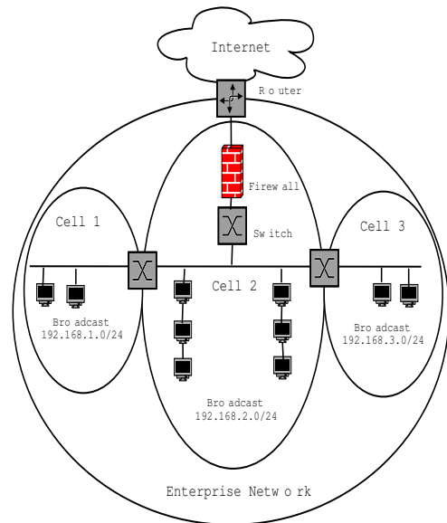
Figure 1. Dividing an Enterprise Network into Cells. Three network cells are separated by switches. Each cell has its own Class C network and distinct broadcast domain.
