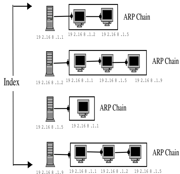
Figure 2. Peer List for a small network with four active devices. There are four ARP chains of 2, 3, 1 and 3 elements. Each ARP chain is comprised of an index value equal to an ARP requestor’s IP address. The index and the associated collection of ARP chains is known collectively as the peer list.
