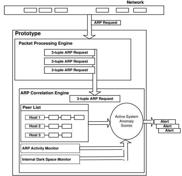
Figure 3. High Level Design of Prototype Implementation
